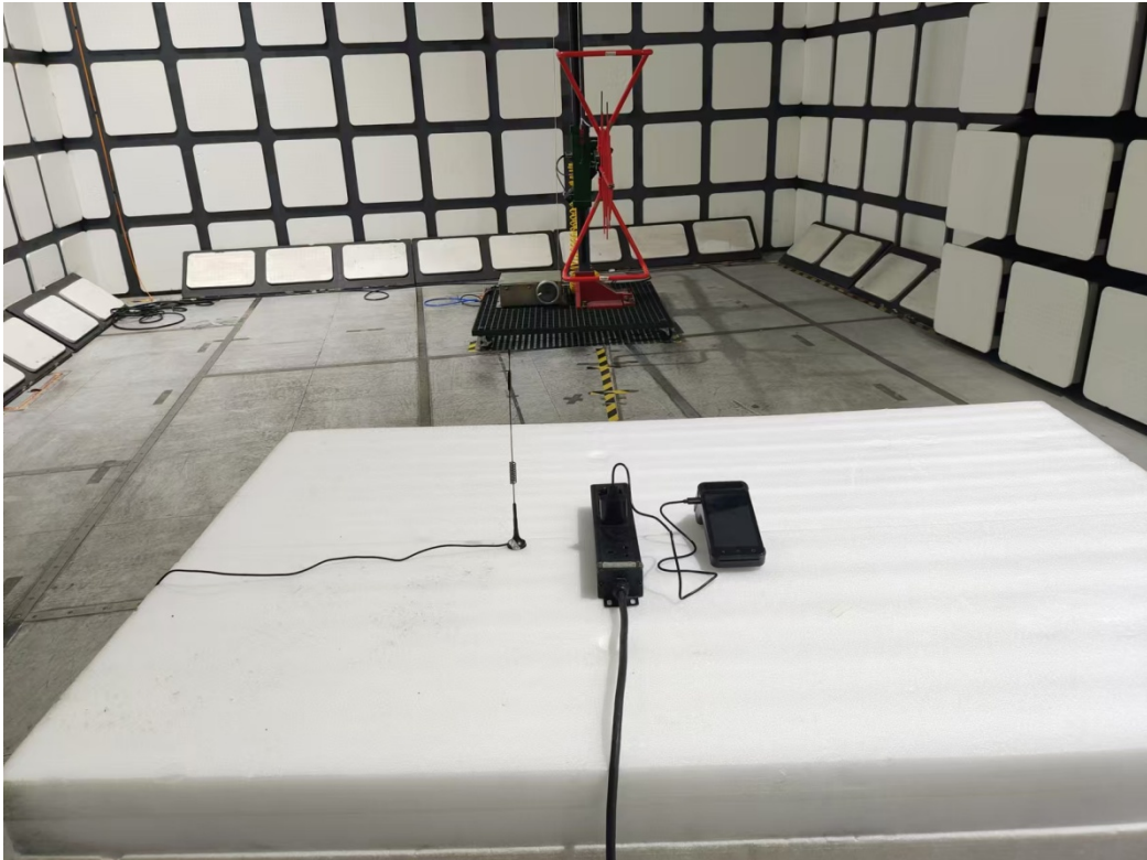
Radiated Emissions View (30MHz-1GHz)
