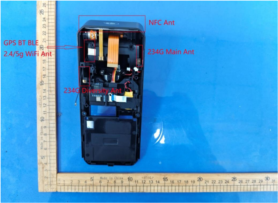
Antenna location diagram
