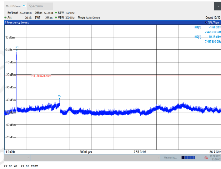
11N40SISO Ant1 2452 0~Reference
