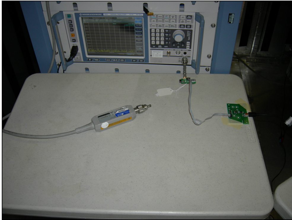
Figure 5: RF Conducted Emissions
