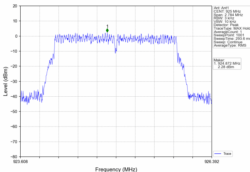
2M_HCH_925MHz_Ant1_NTNV
