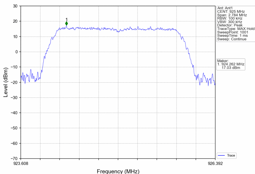
2M_HCH_925MHz_Ant1_NTNV
