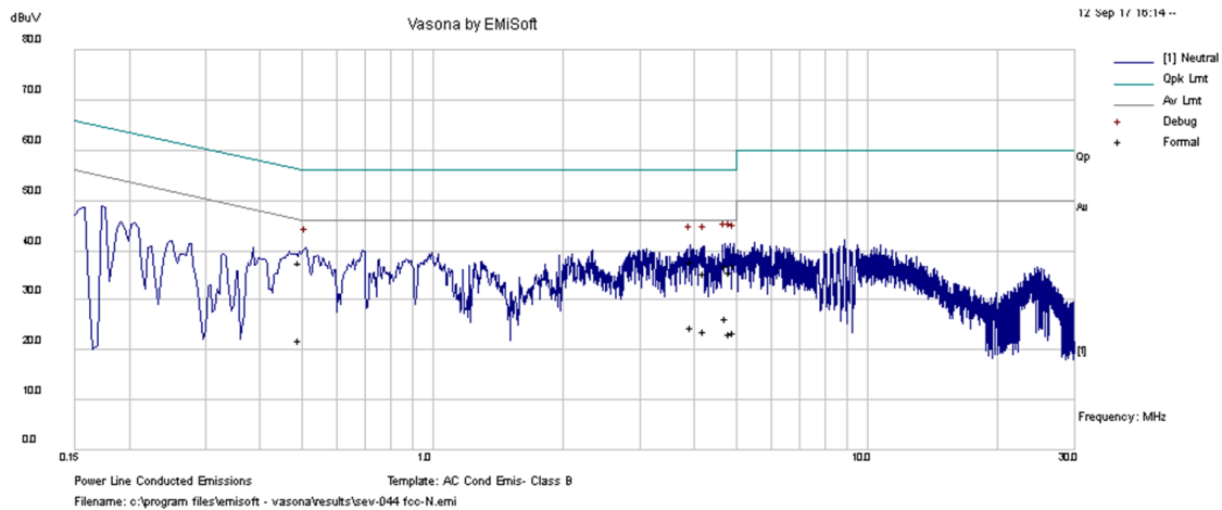
Neutral Plot at 120Vac, 60Hz
