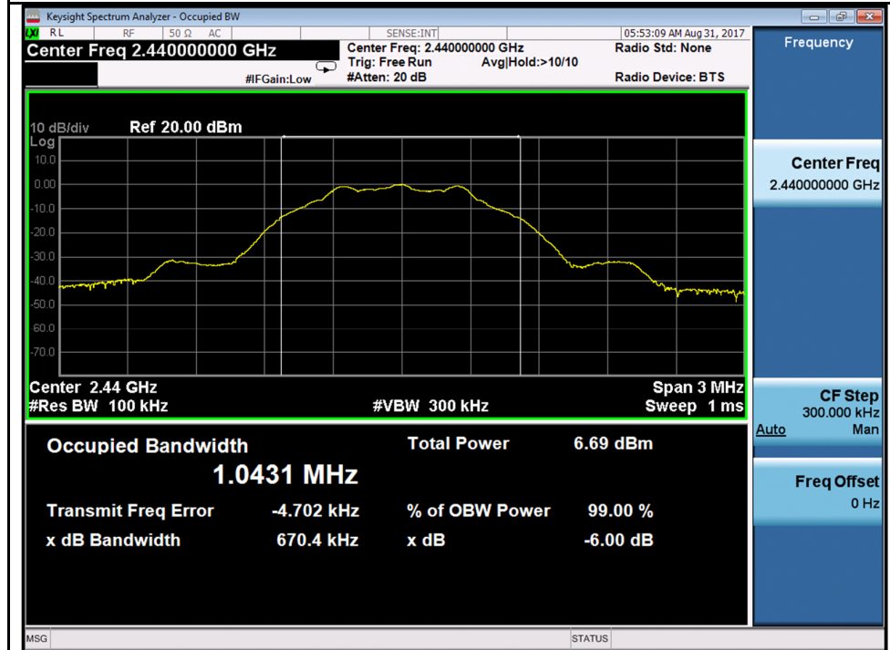
BLE-2440MHz
