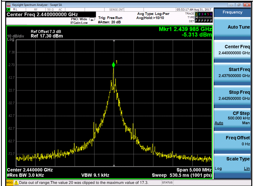
BLE-2440MHz
