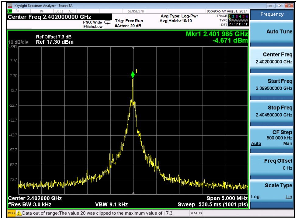
BLE-2402MHz
