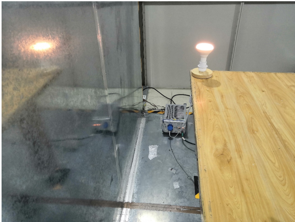
Conducted Emissions -Left View
