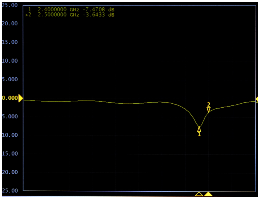
SWR test chart
