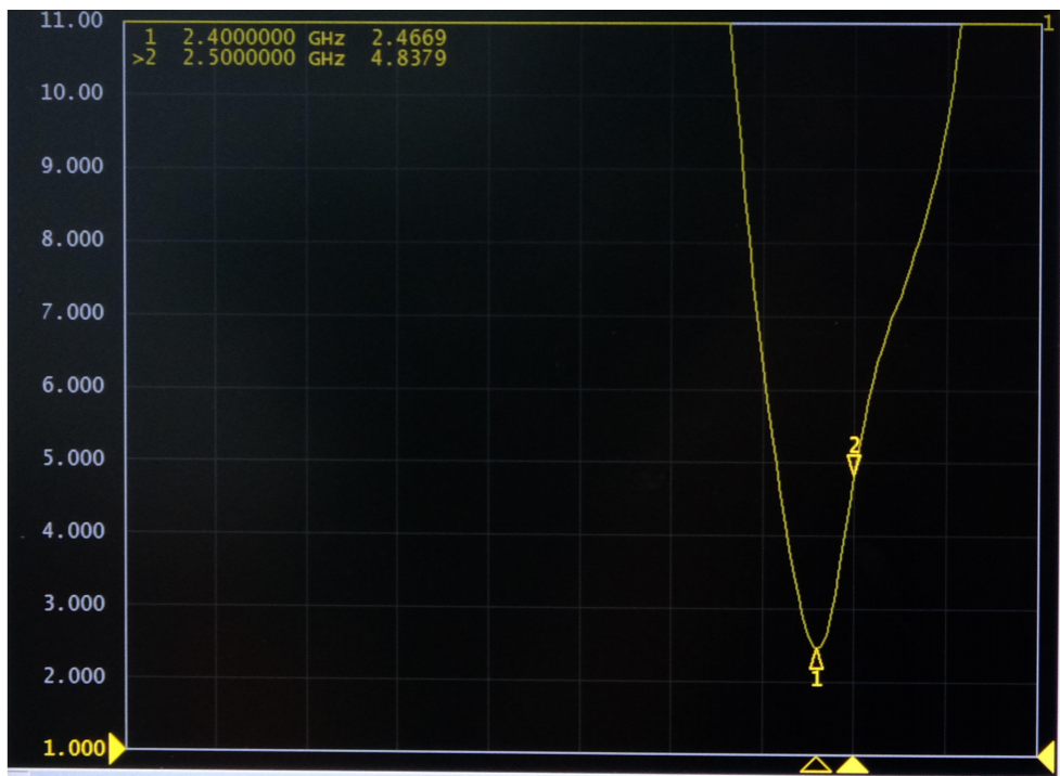
SWR test chart
