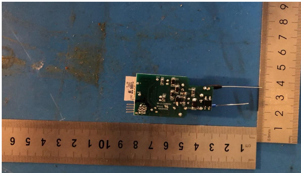
MAIN BOARD TOP VIEW (EBE-QPW113-F)
