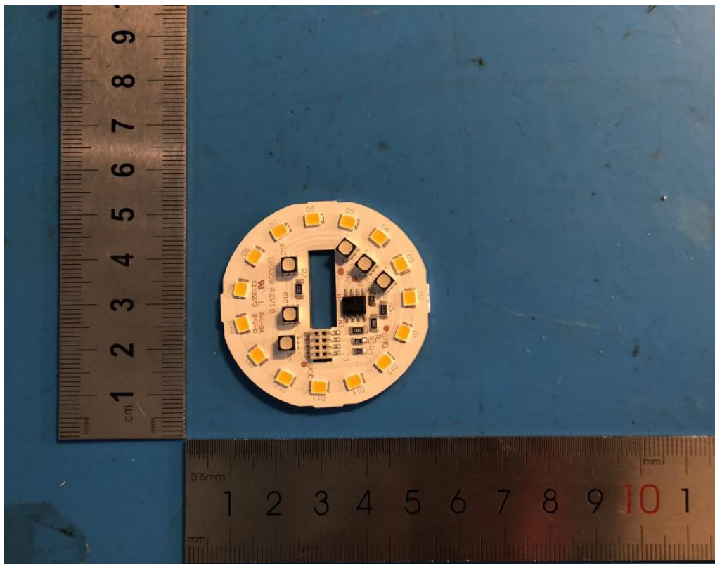
MAIN BOARD TOP VIEW (EBE-QPW113-F)
