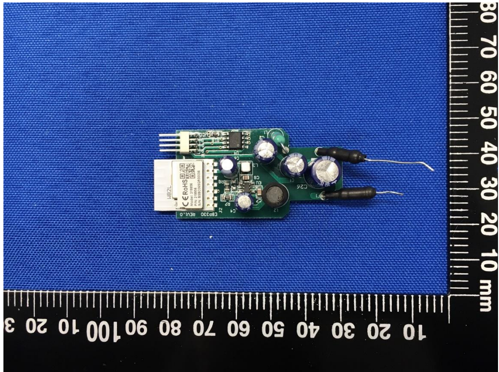
MAIN BOARD REAR VIEW (EBE-QPW113)
