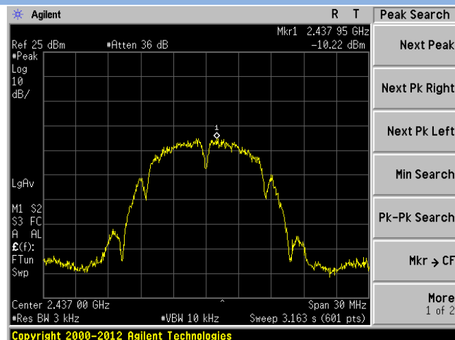
802.11b CHANNEL 6
