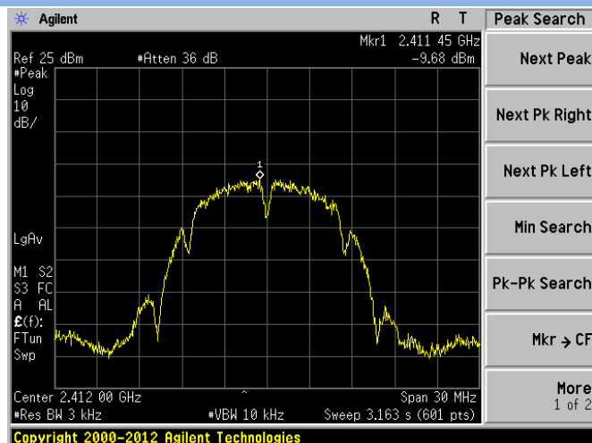
802.11b CHANNEL 1
