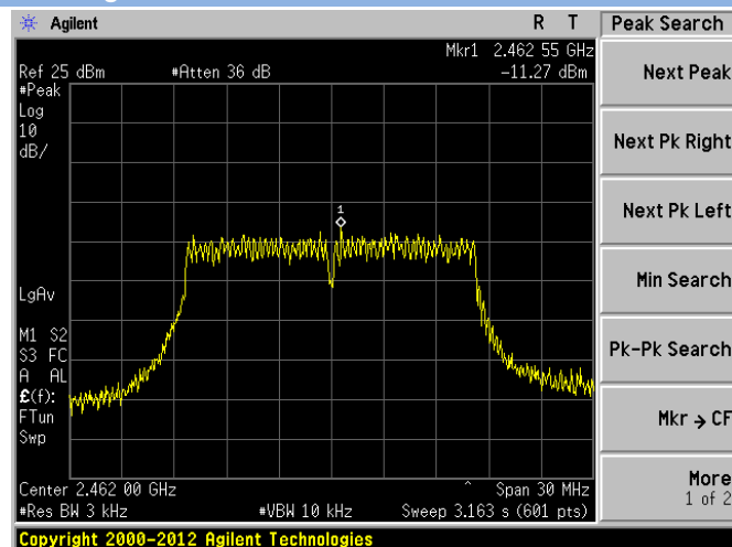
802.11g CHANNEL 11
