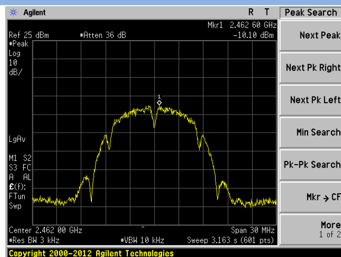
802.11b CHANNEL 11
