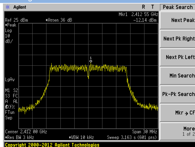
802.11g CHANNEL 1
