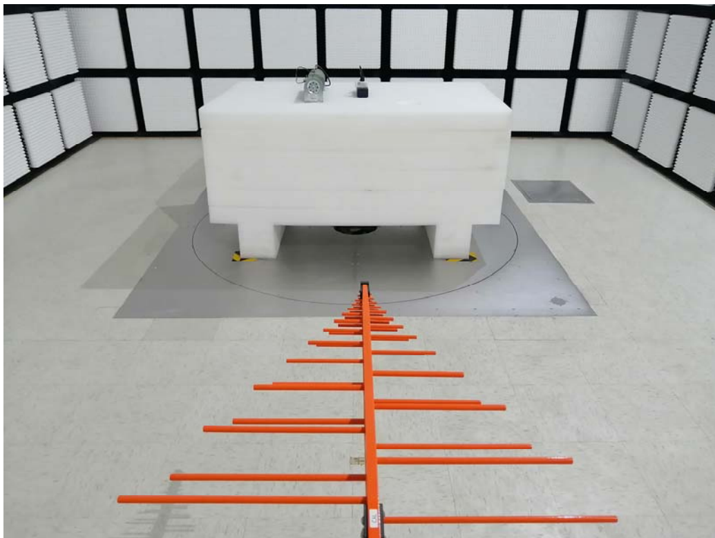
Radiated Emissions Below 1G View EBE-SW010-A
