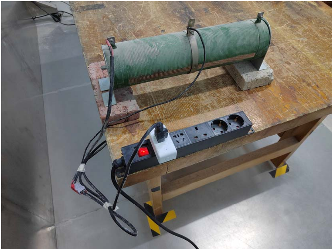
Conducted Emissions Side View EBE-SW010
