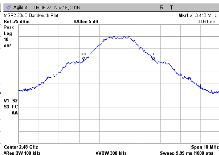
MSP2; 2480 MHz
