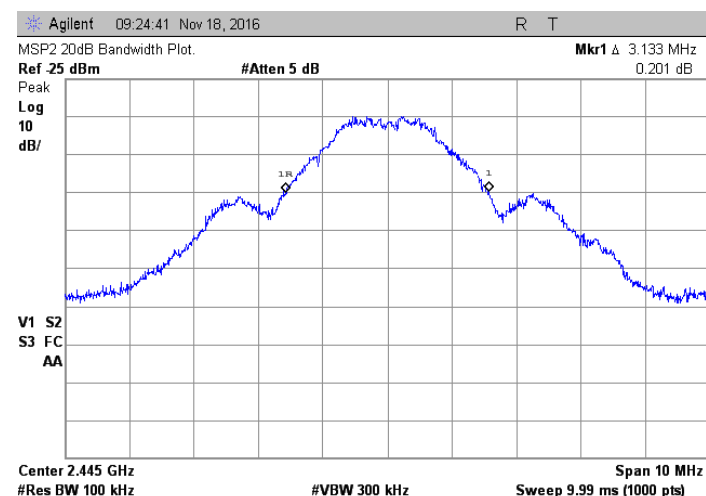
MSP2; 2445 MHz
