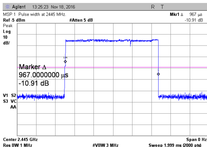
MSP1 Duty Cycle
