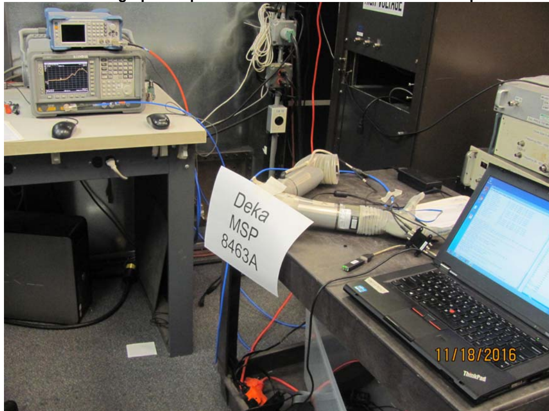
Photograph of Spurious Conducted Emissions Test Setup
