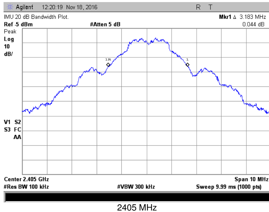
Figure 2. Occupied Bandwidth Plots
