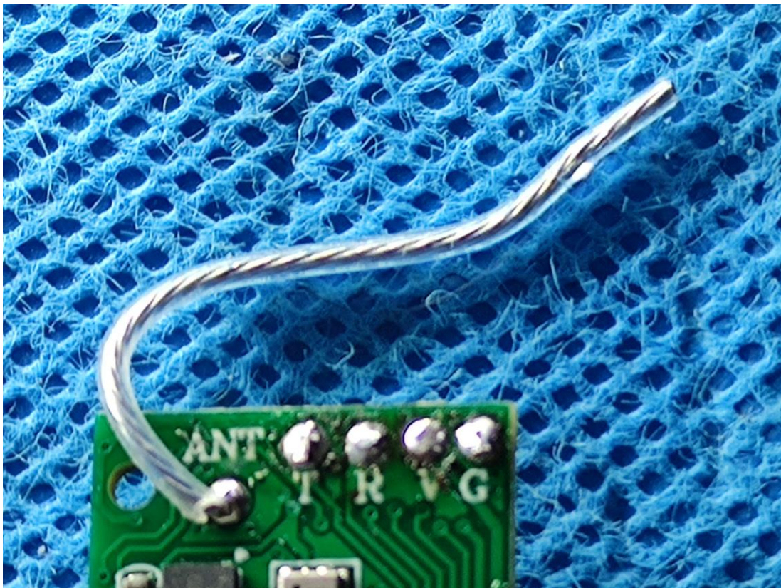
SRD Receive Antenna
