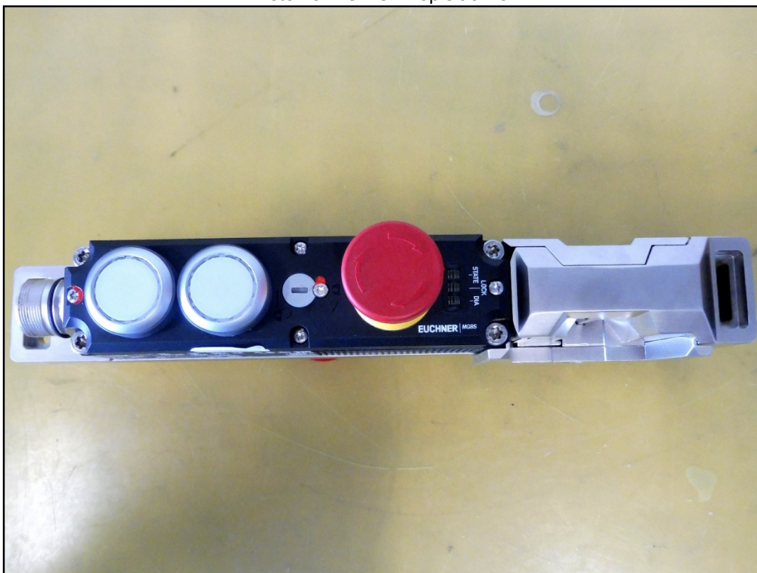
Photo 13: DUT C - Top side view
