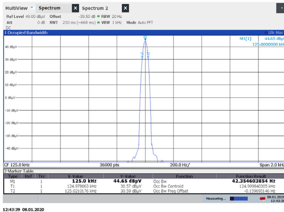
Plot 1: 99 % emission bandwidth without tag
