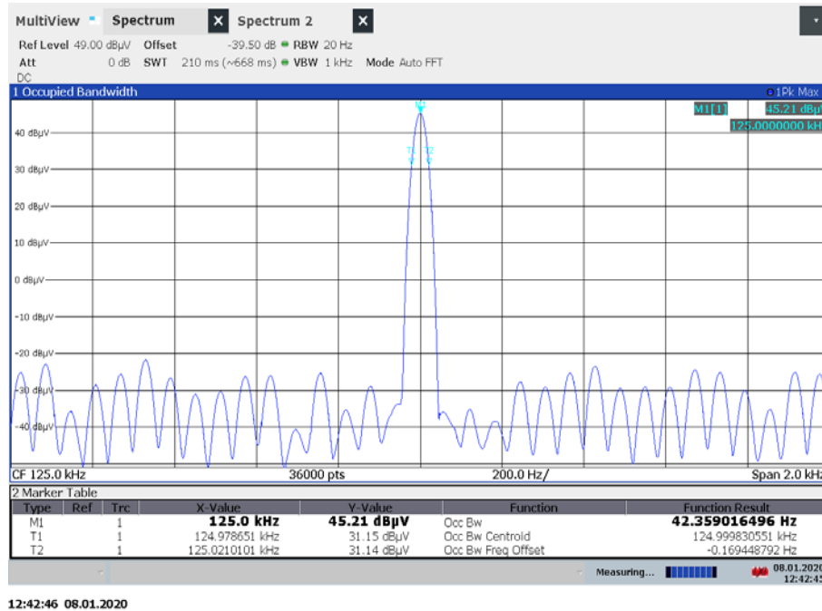
Plot 1: 99 % emission bandwidth with applied tag
