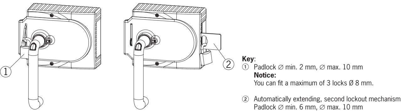
Figure 5: Lockout mechanism secured with padlock
