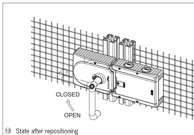
Figure 13: Changing actuating direction, final state
