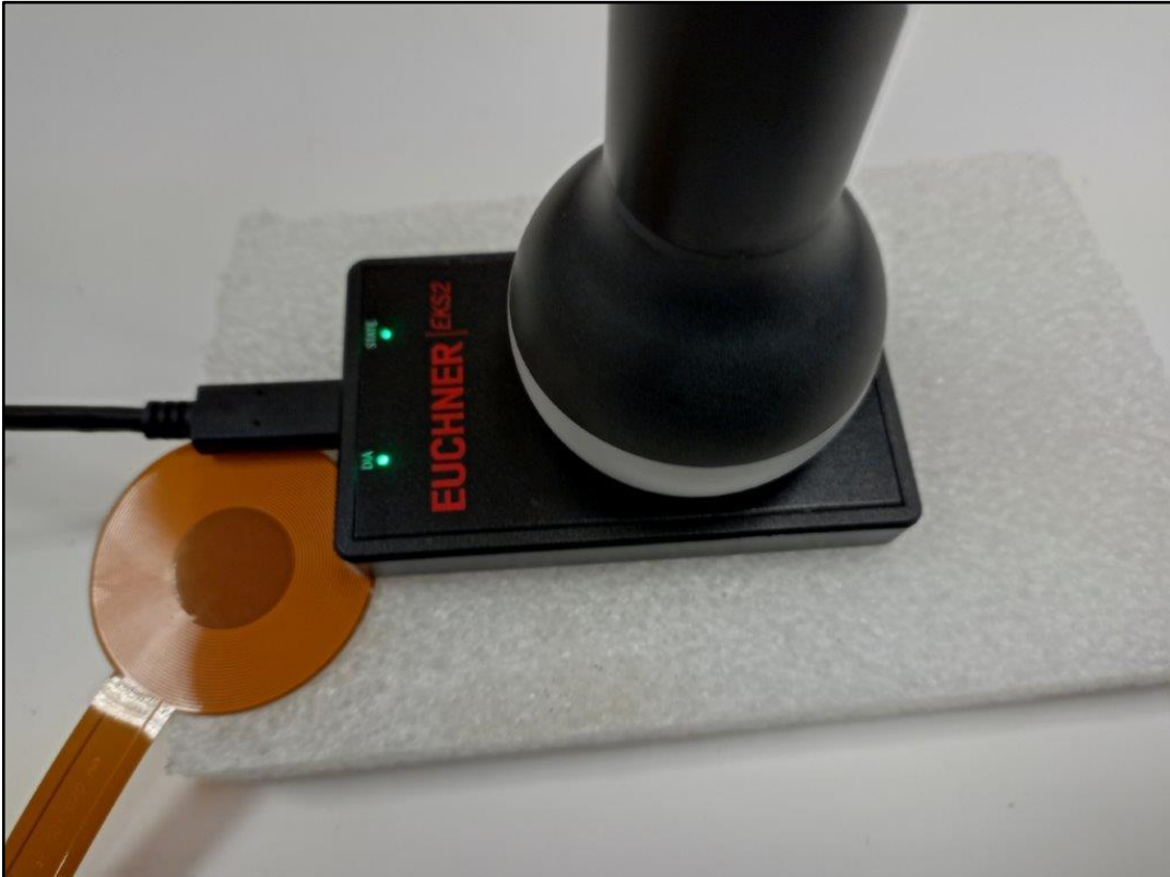
Photo 6: EUT – Test Setup (position – back)
