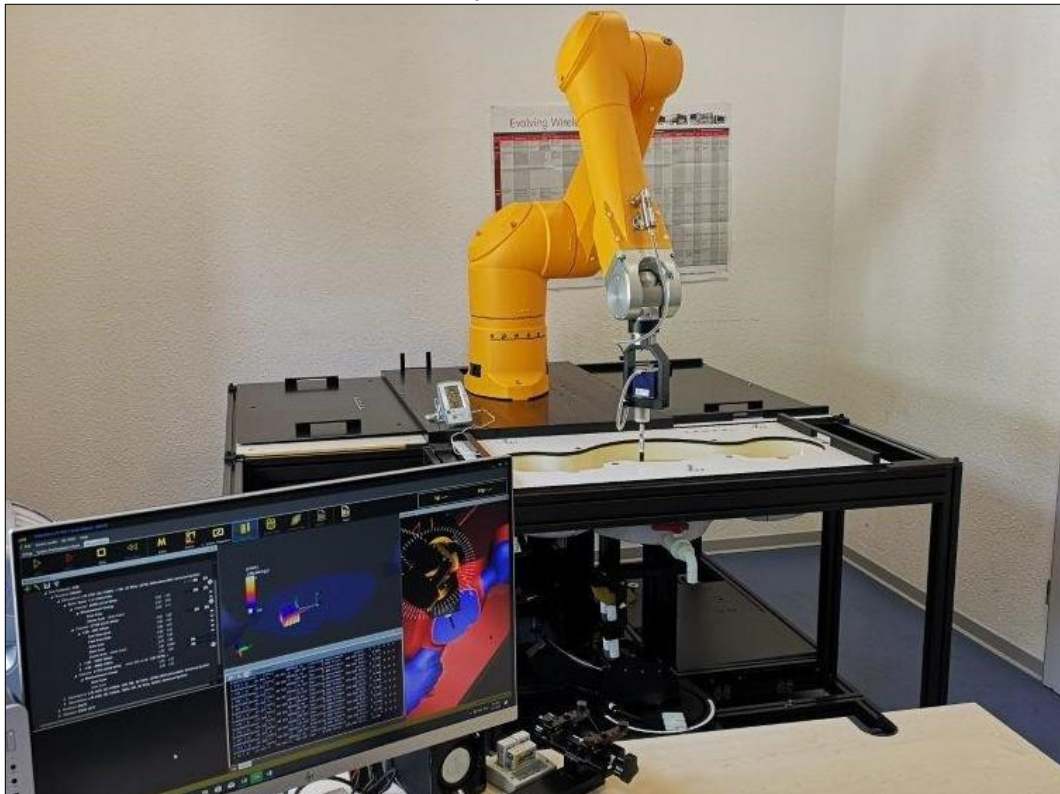
Photo 2: Measurement System DASY, SAR 4 MHz to 6 GHz
