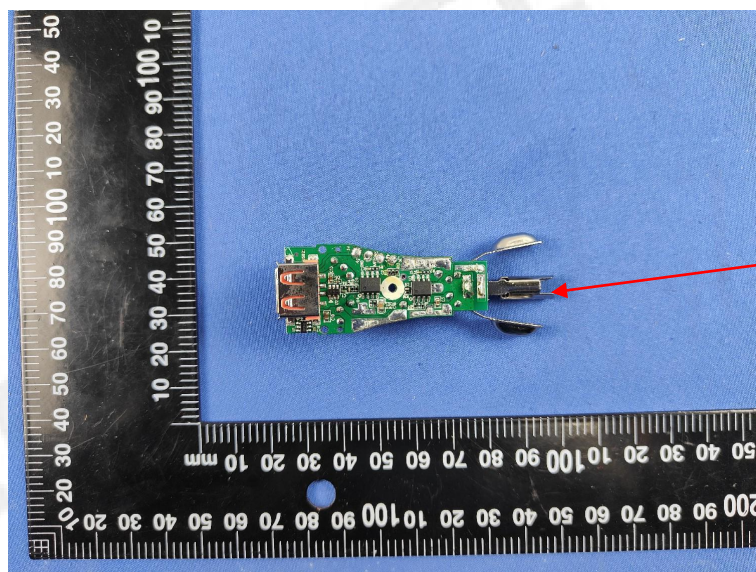
FM Antenna
