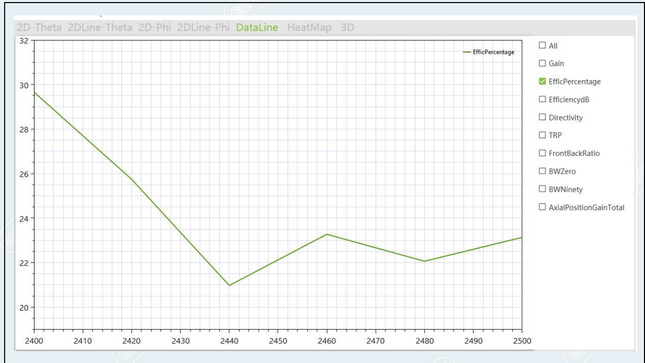
Efficiency plot
