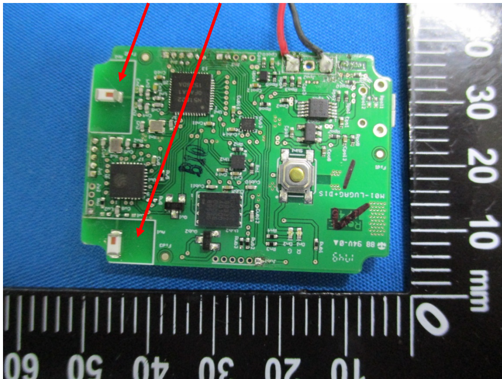
BLE and Wi-Fi Antenna Location
