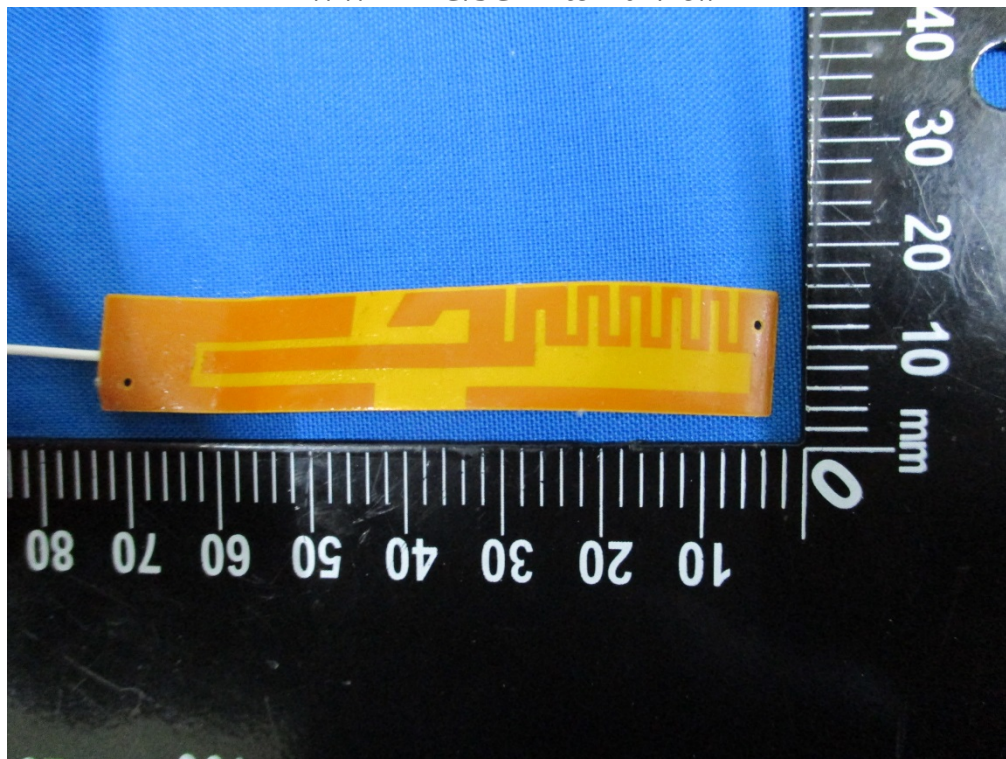
WWAN 2G/3G Antenna View
