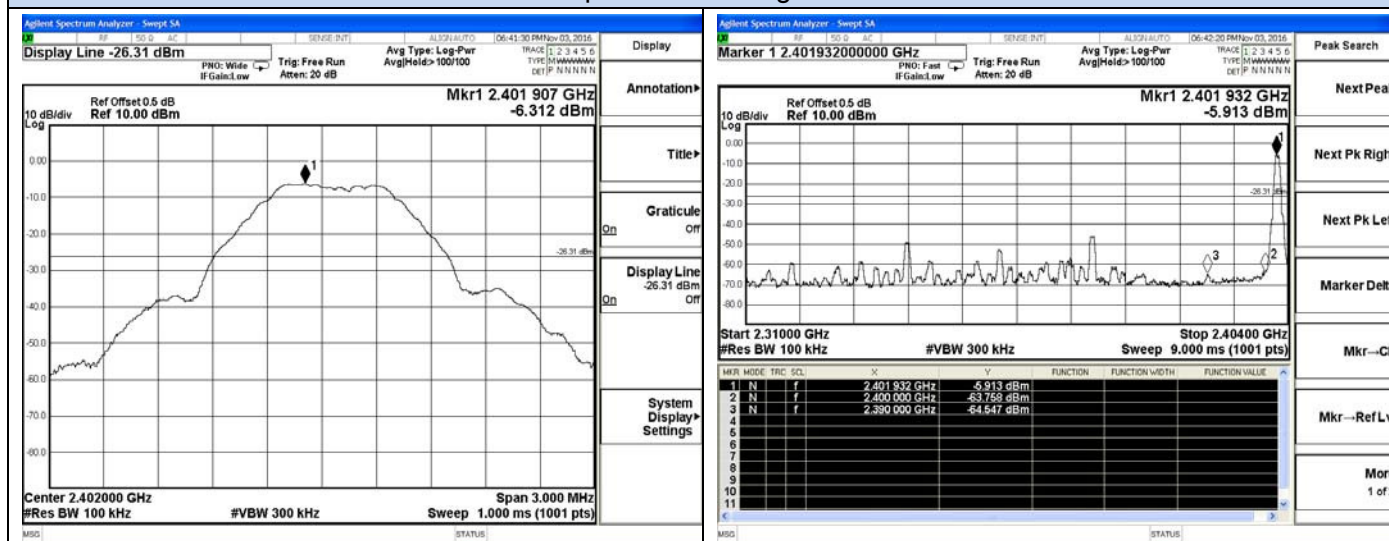
BT LE-Low channel Reference
