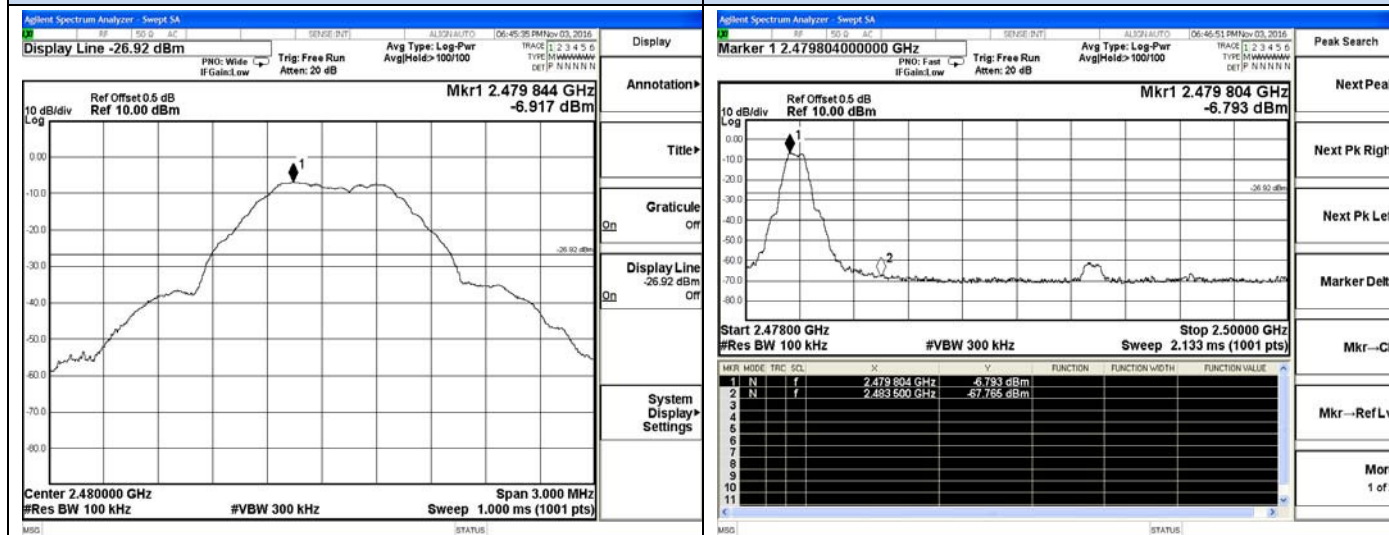
BT LE-High channel Reference
