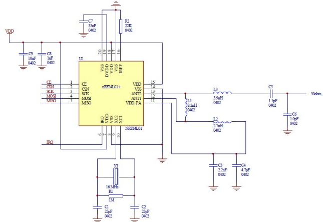
Figure 32. nRF24L01+ schematic for RF layouts with single ended 50Ω RF output
