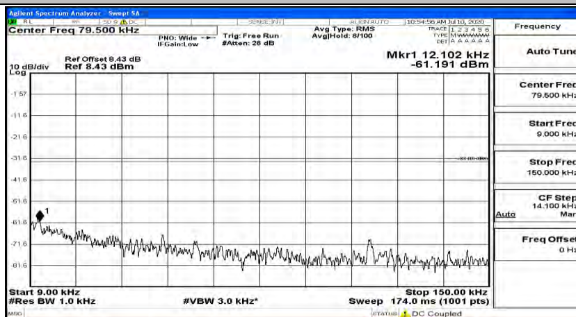
CSE Test Graph(s) (Channel Bandwidth: 5 MHz)_HCH_QPSK
