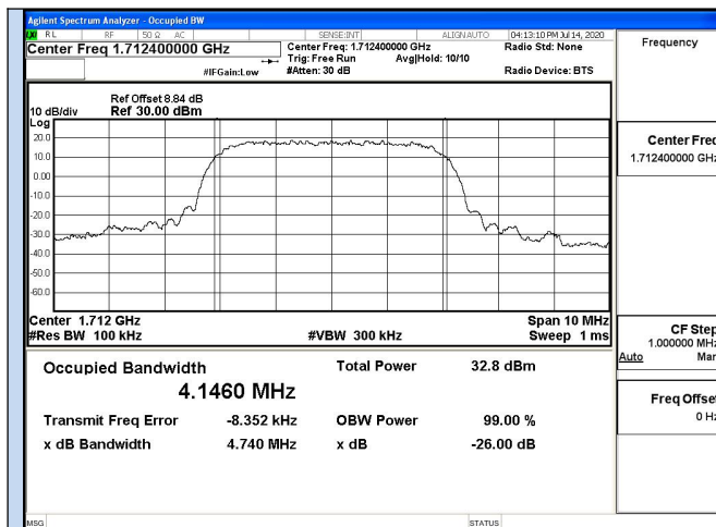
Channel 1312 / 1712.4 MHz
