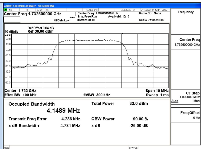
Channel 1413 / 1732.6 MHz
