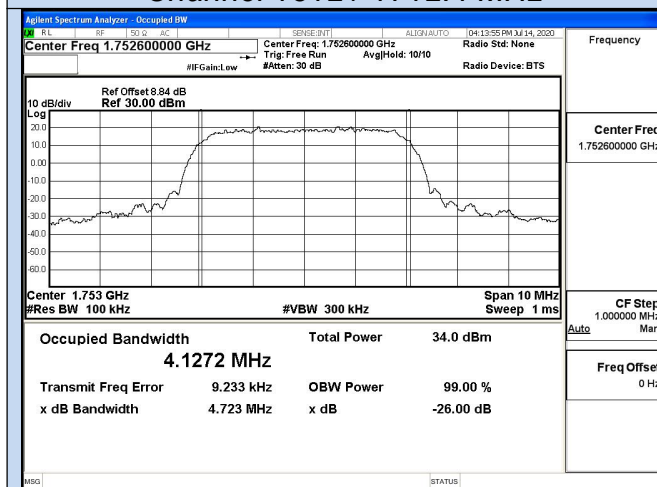
Channel 1513 / 1752.6 MHz
