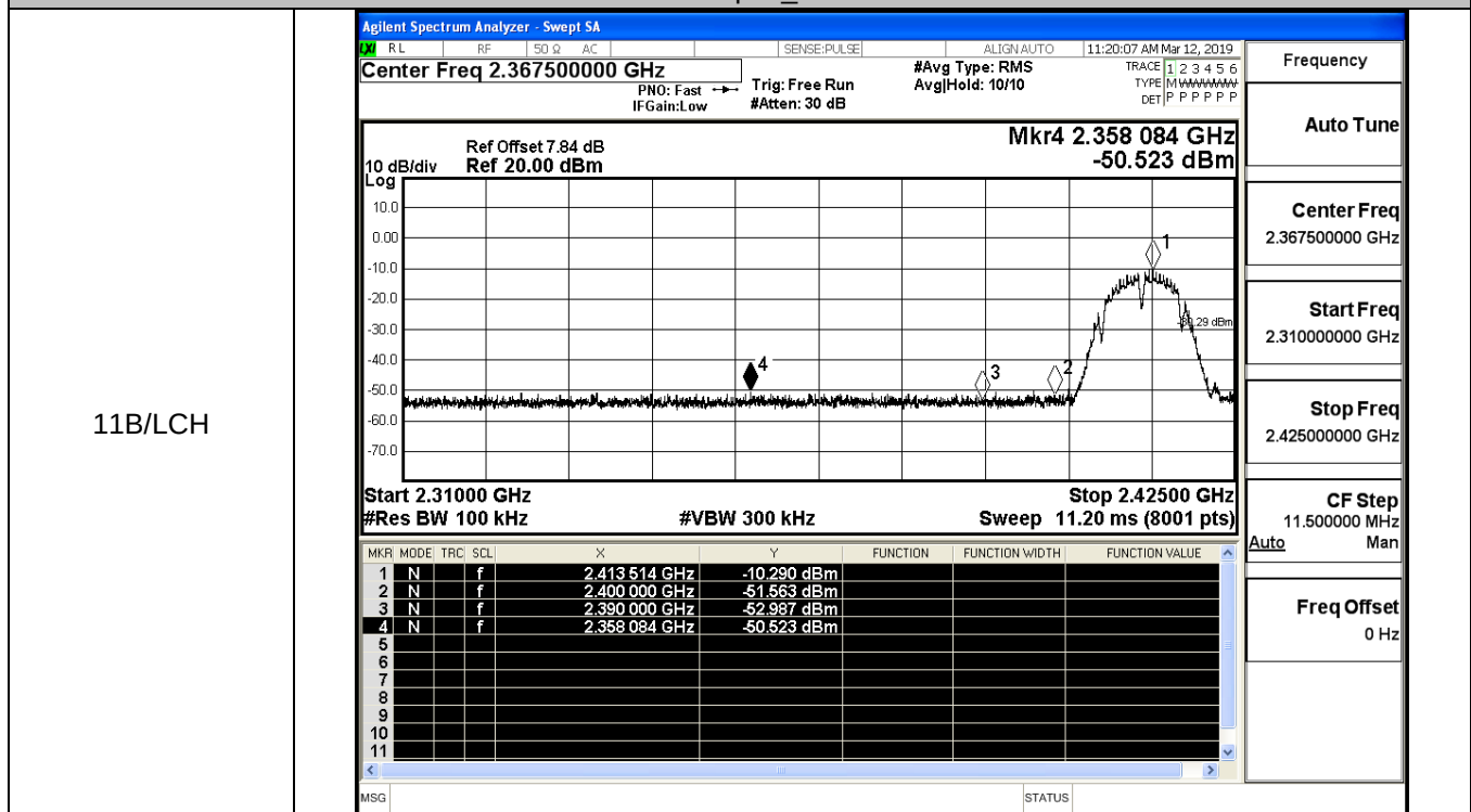
Test Graphs_Ant0
