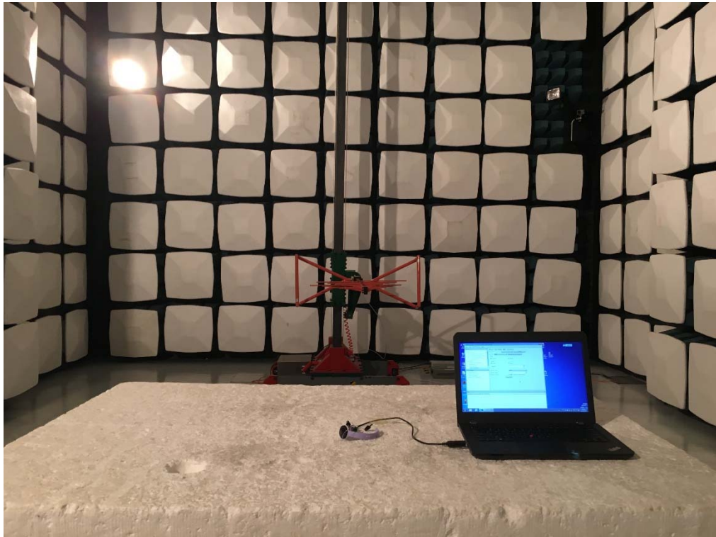
Radiated emission Test Setup-1(Below 1GHz)
