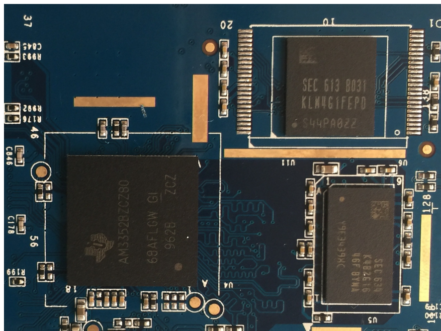
EUT – PCB-2 Main chips View-1
