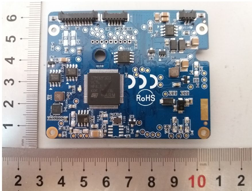
EUT – PCB-1 Main chips View-1
