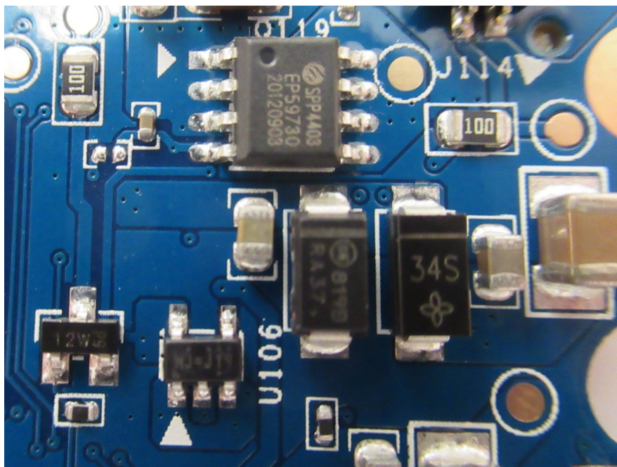
EUT – PCB-1 Main chips View-3
