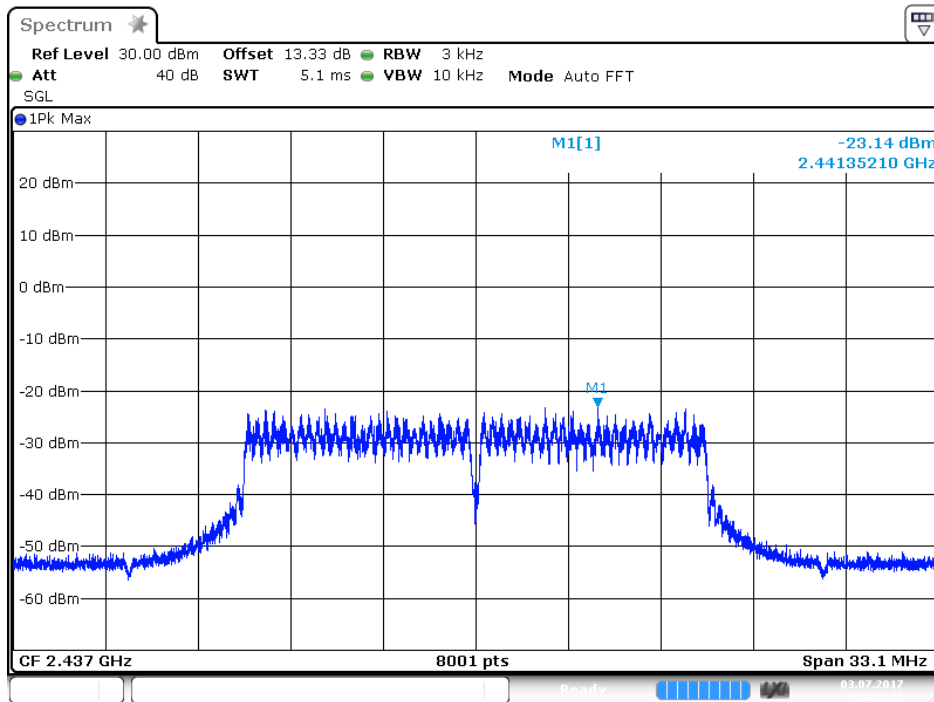
802.11g - Channel 6
