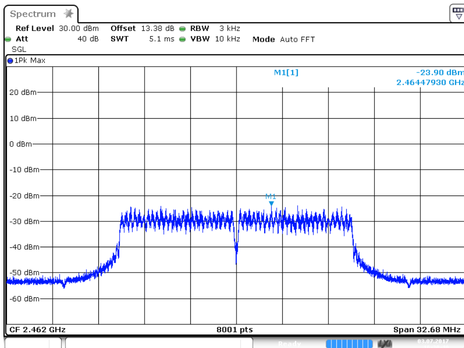
802.11g - Channel 11
