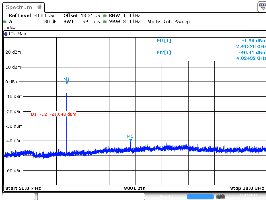
802.11b - Conducted Spurious Emission Plot on channel 1
