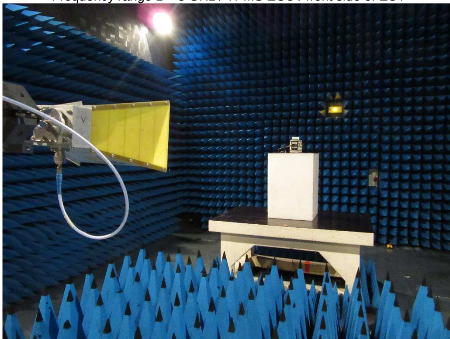
Frequency range 1 – 3 GHz / TPMS ECU / front side of EUT
