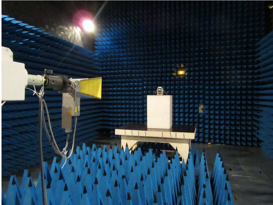
Frequency range 3 – 18 GHz / TPMS ECU / front side of EUT
