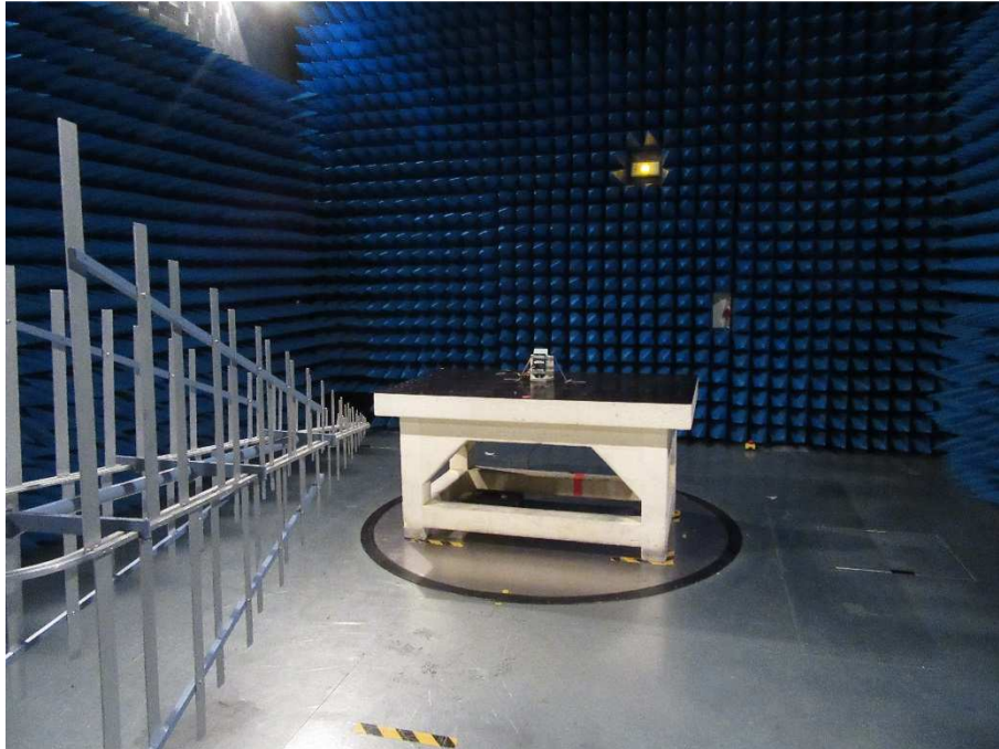
TPMS ECU / front side of EUT
