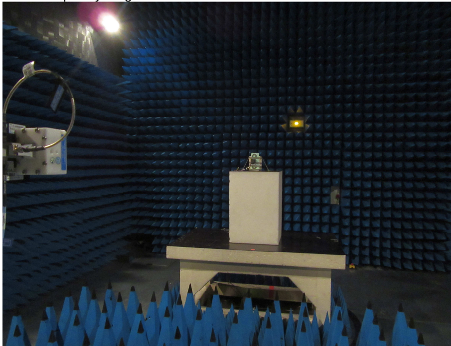
Frequency range 18 – 26.5 GHz / TPMS ECU / front side of EUT
