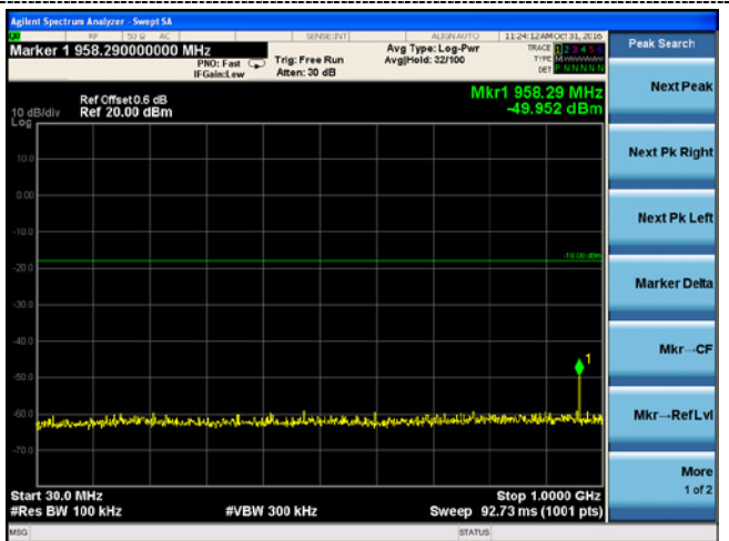
30MHz~1GHz
