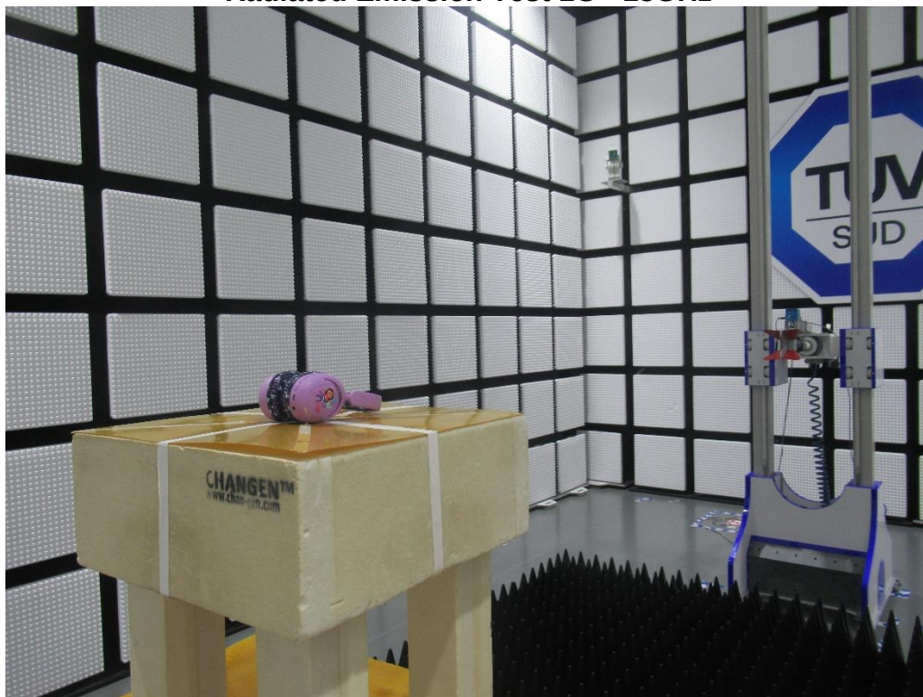
Radiated Emission Test 1G - 18GHz
