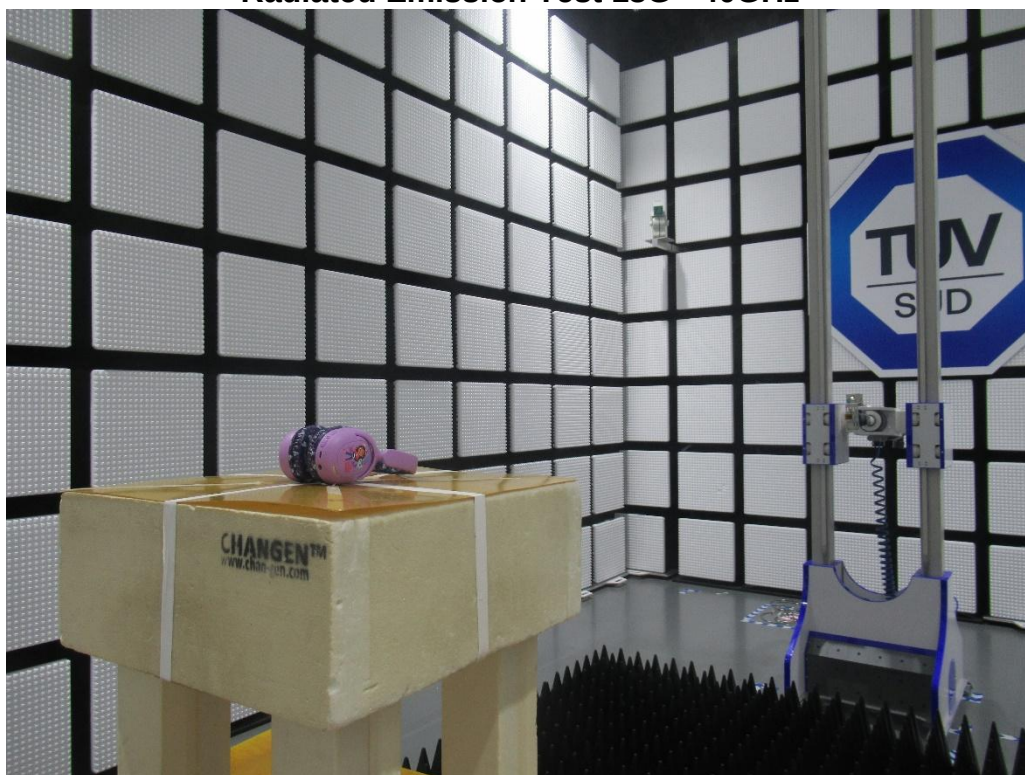
Radiated Emission Test 18G - 40GHz
