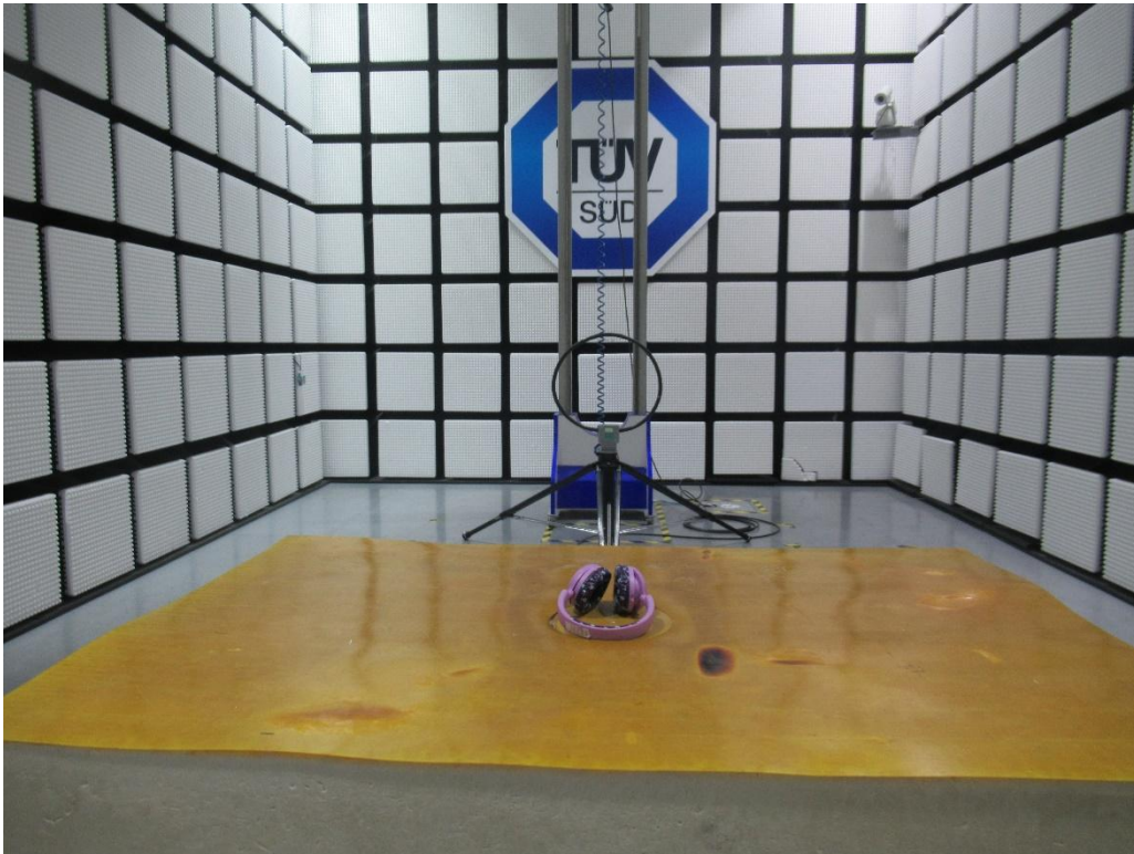
Radiated Emission Test 9k - 30MHz
