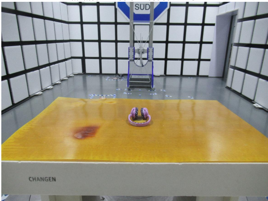
Radiated Emission Test 30M - 1GHz
