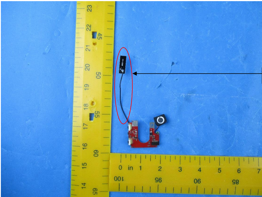
RF Antenna
