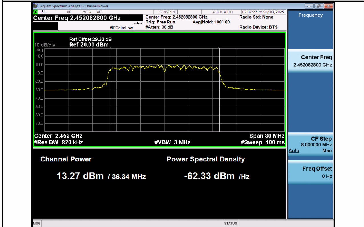
11N40SISO-Ant1-2452-PASS
