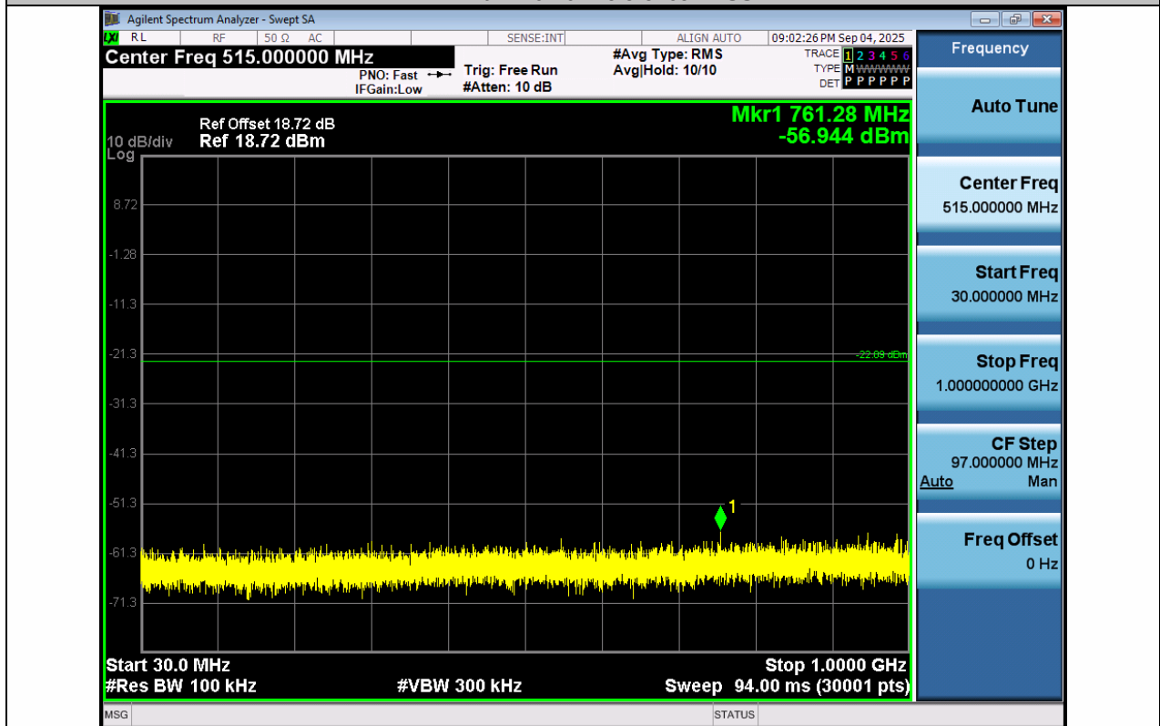
11B-Ant1-2462-30~1000-PASS
