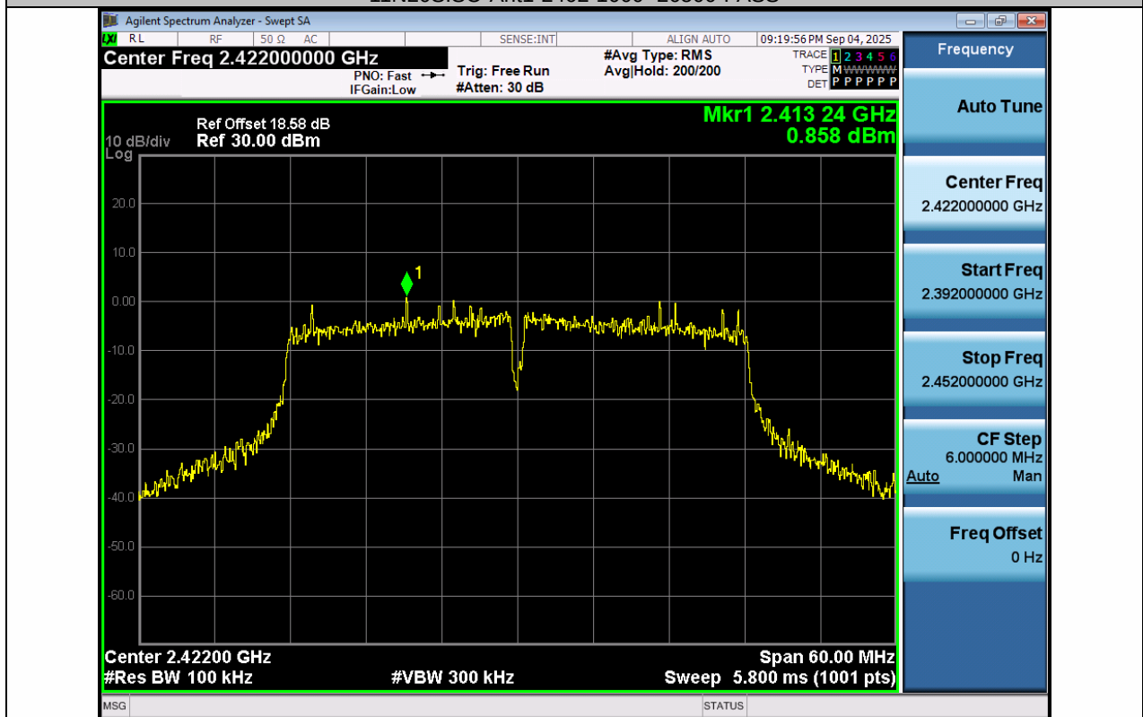
11N40SISO-Ant1-2422-0-Reference-PASS
