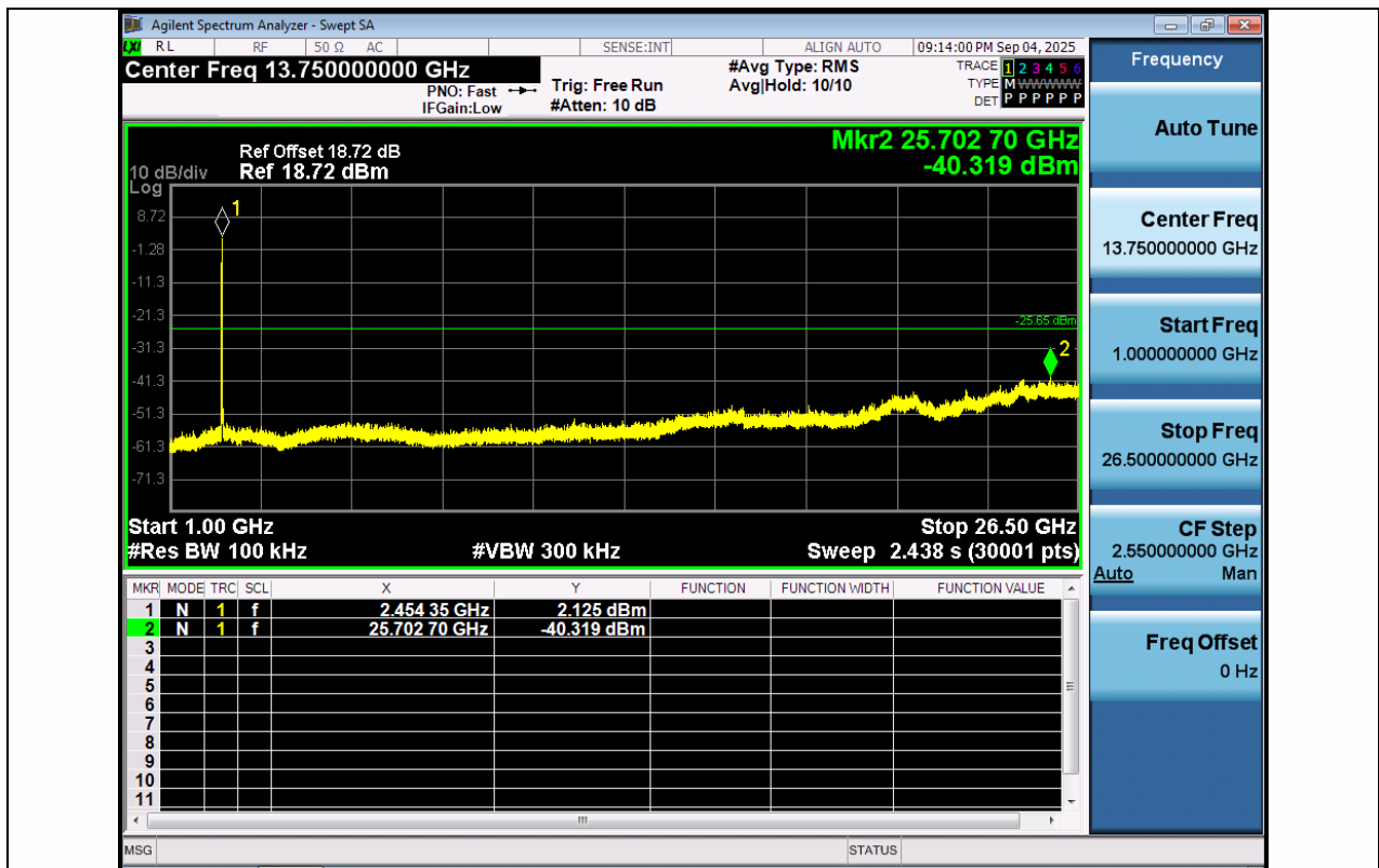
11N20SISO-Ant1-2462-1000-26500-PASS
