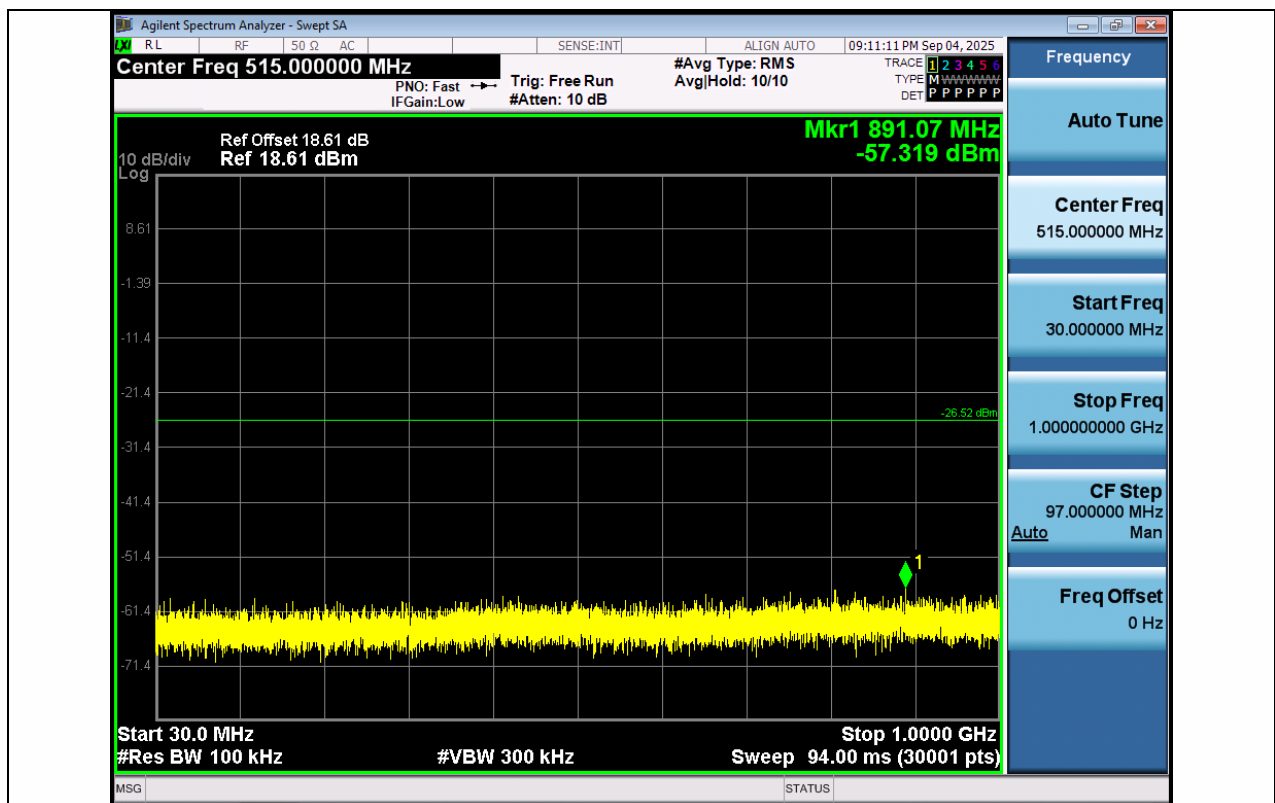
11N20SISO-Ant1-2437-30~1000-PASS
