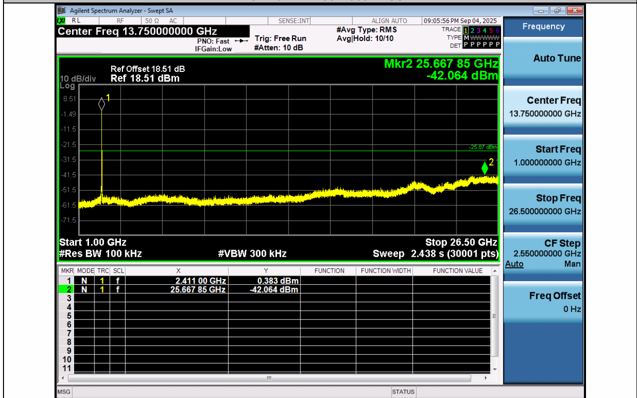
11G-Ant1-2412-1000-26500-PASS
