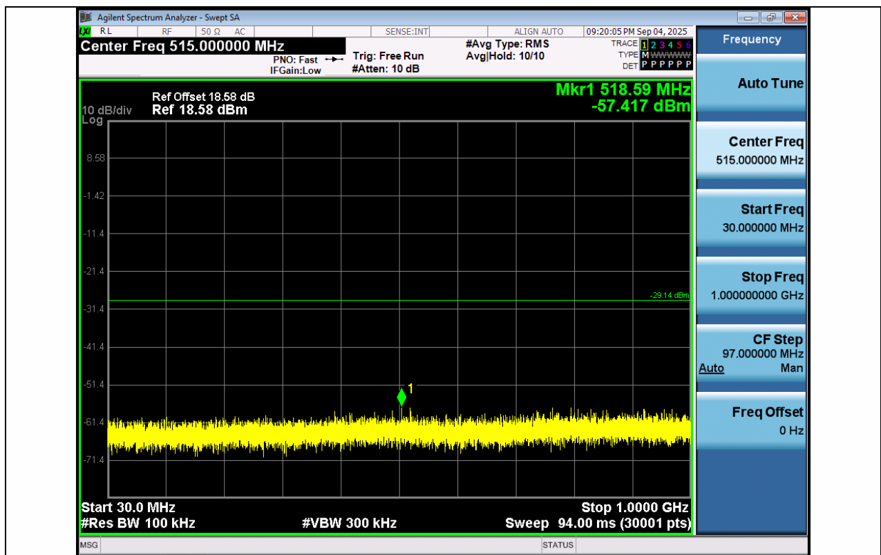
11N40SISO-Ant1-2422-30~1000-PASS
