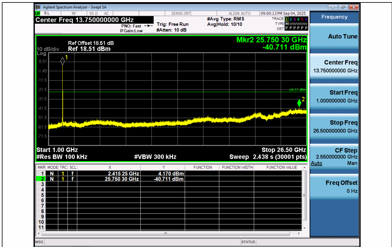
11B-Ant1-2412-1000~26500-PASS
