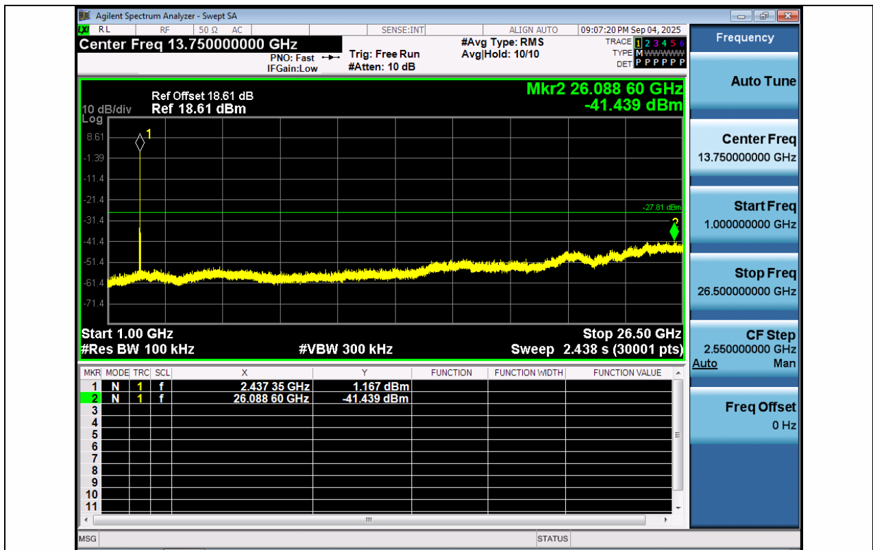
11G-Ant1-2437-1000~26500-PASS
