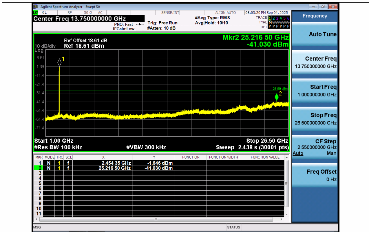
11N40SISO-Ant1-2437-1000-26500-PASS
