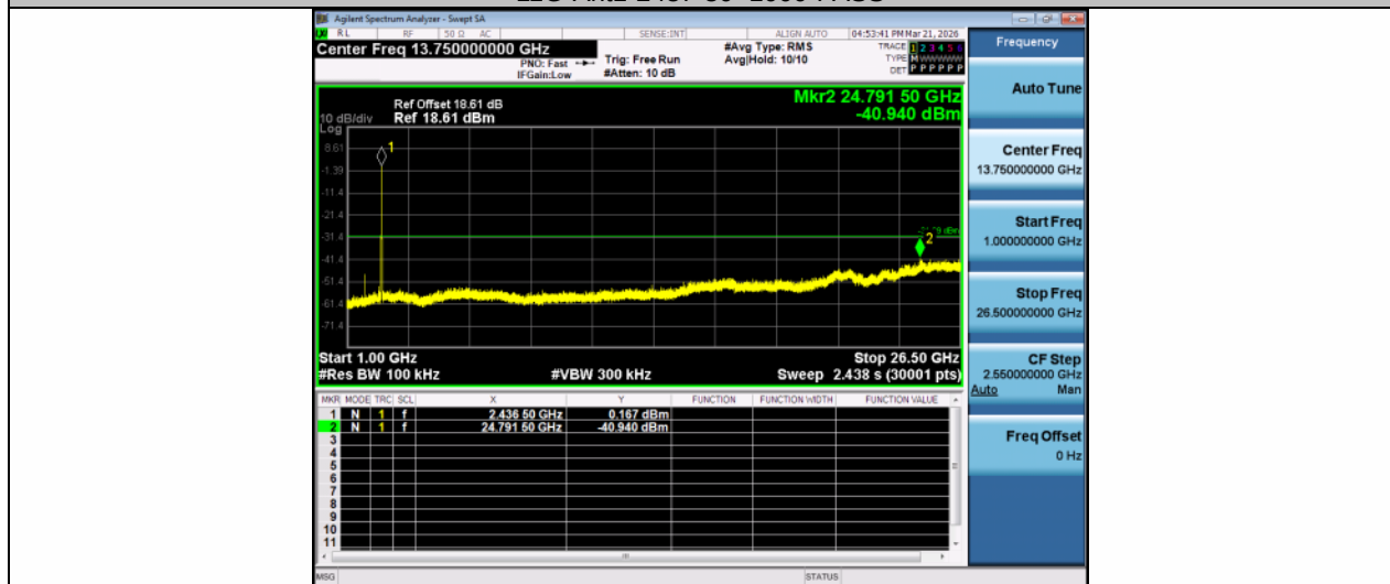
11G-Ant1-2437-1000~26500-PASS
