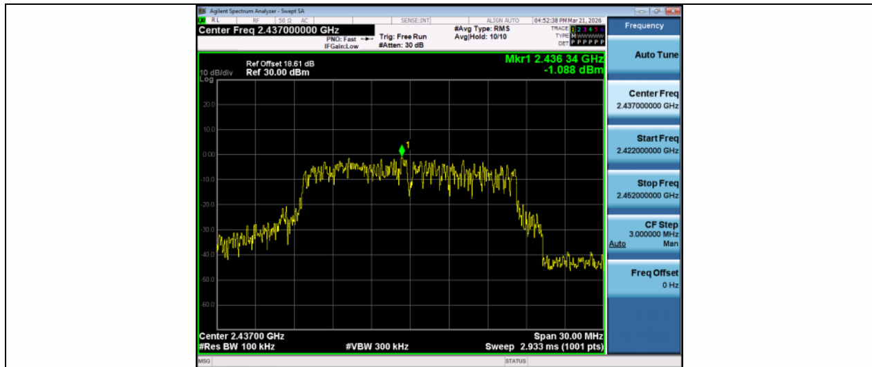
11G-Ant1-2437-0~Reference-PASS
