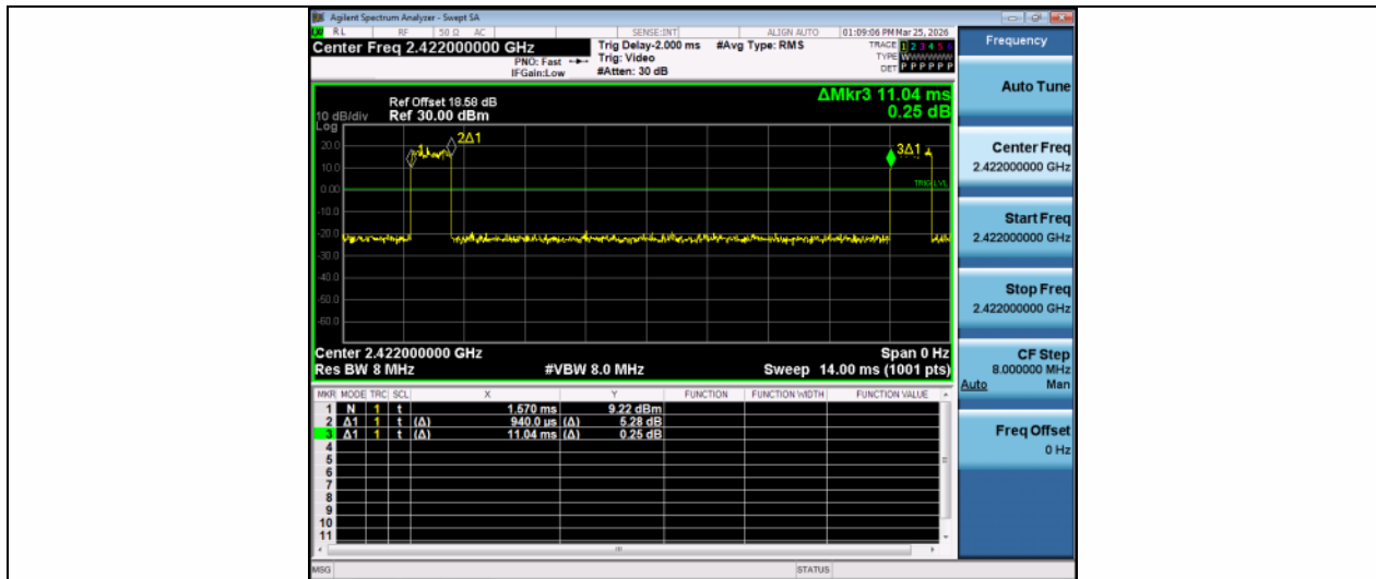
NTNV-11N40SISO-Ant1-2422
