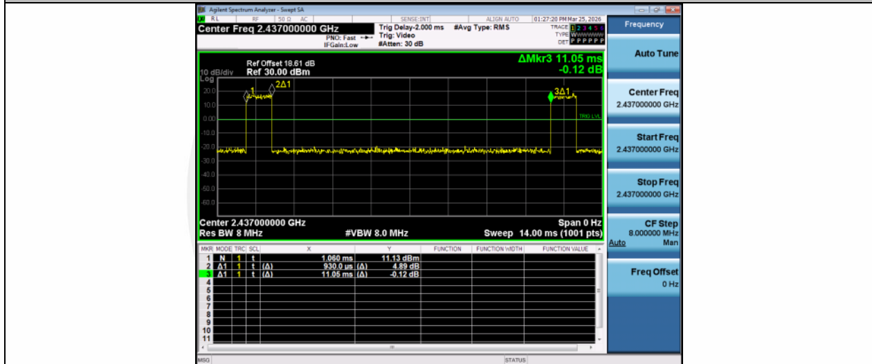
NTNV-11N40SISO-Ant1-2437
