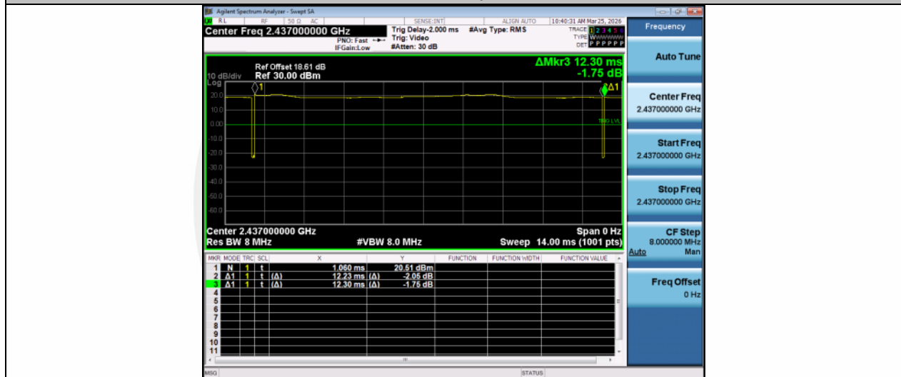
NTNV-11B-Ant1-2437
