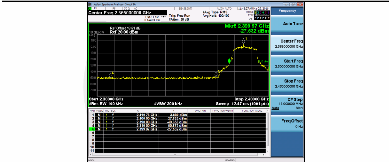
11N20SISO-Ant1-2412-PASS
