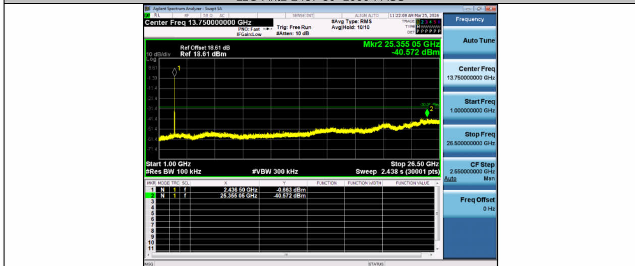
11G-Ant1-2437-1000~26500-PASS
