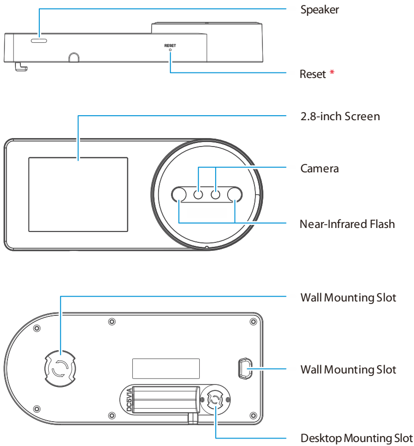
Figure 1-1 Product Appearance
