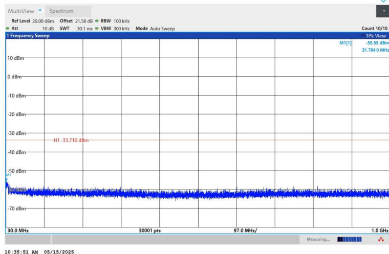
11B-Ant1-2437-30~1000-PASS
