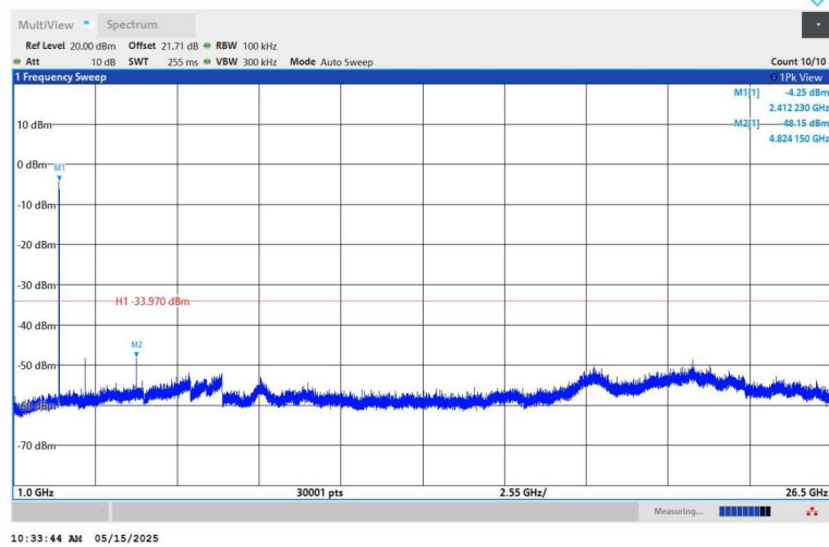
11B-Ant1-2412-1000~26500-PASS
