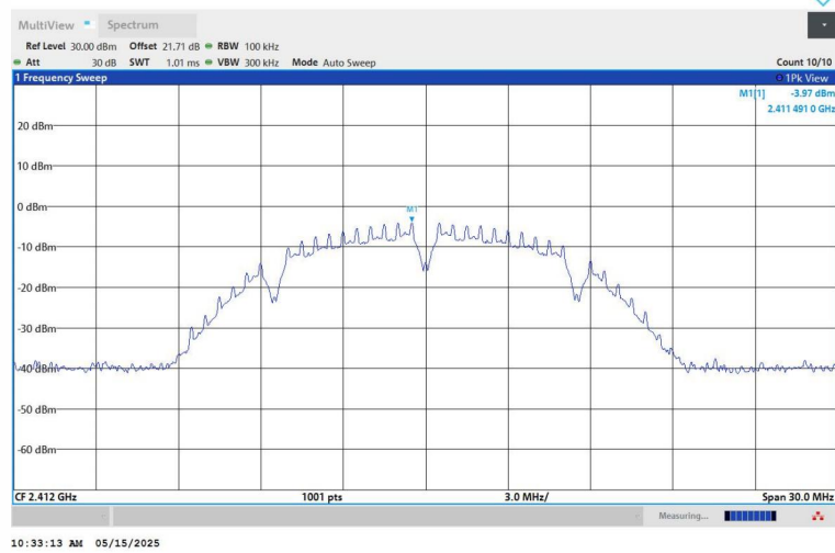
11B-Ant1-2412-0~Reference-PASS
