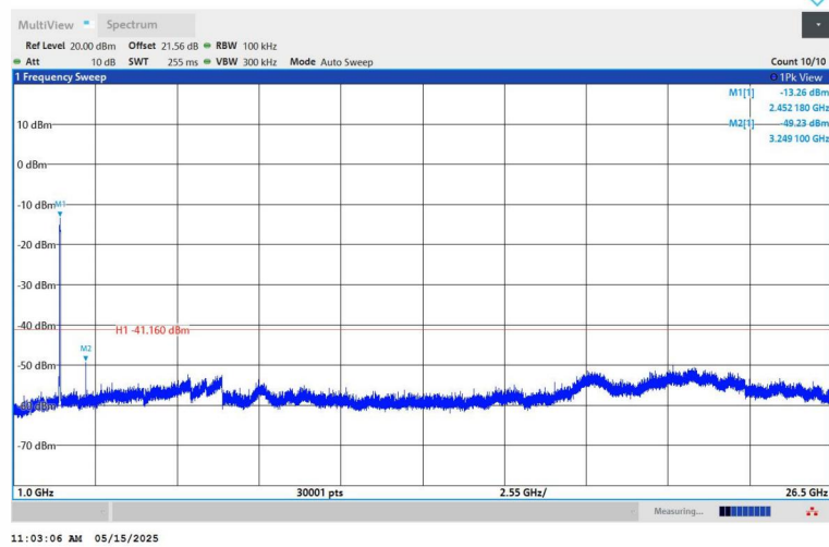
11N40SISO-Ant1-2437-1000~26500-PASS
