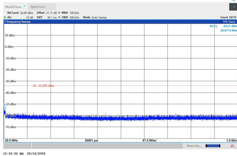
11B-Ant1-2412-30~1000-PASS
