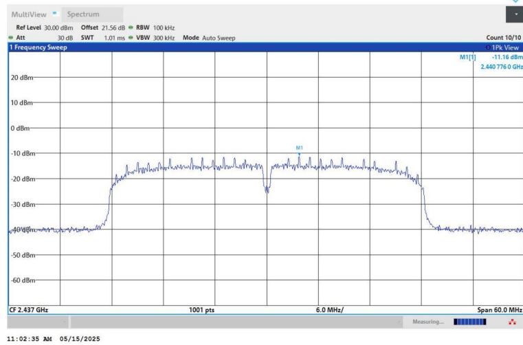
11N40SISO-Ant1-2437-0~Reference-PASS
