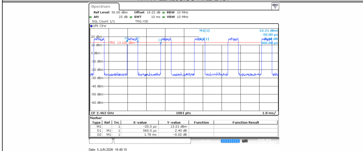
NTNV-11N20SISO-Ant1-2462
