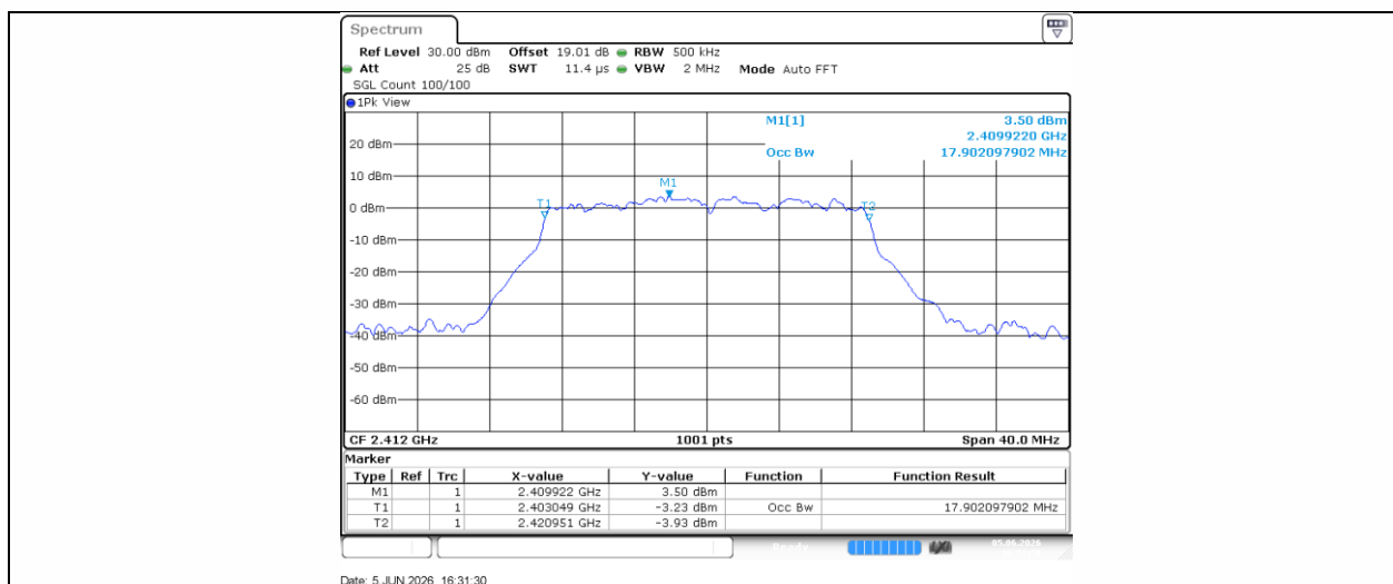
11N20SISO-Ant1-2412
