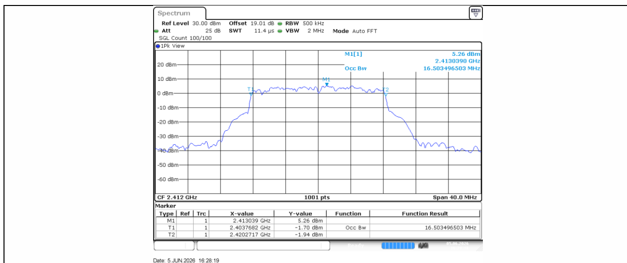
11G-Ant1-2412
