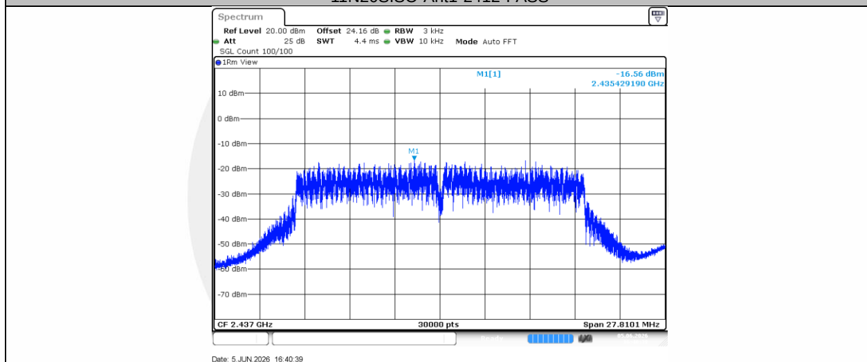
11N20SISO-Ant1-2437-PASS
