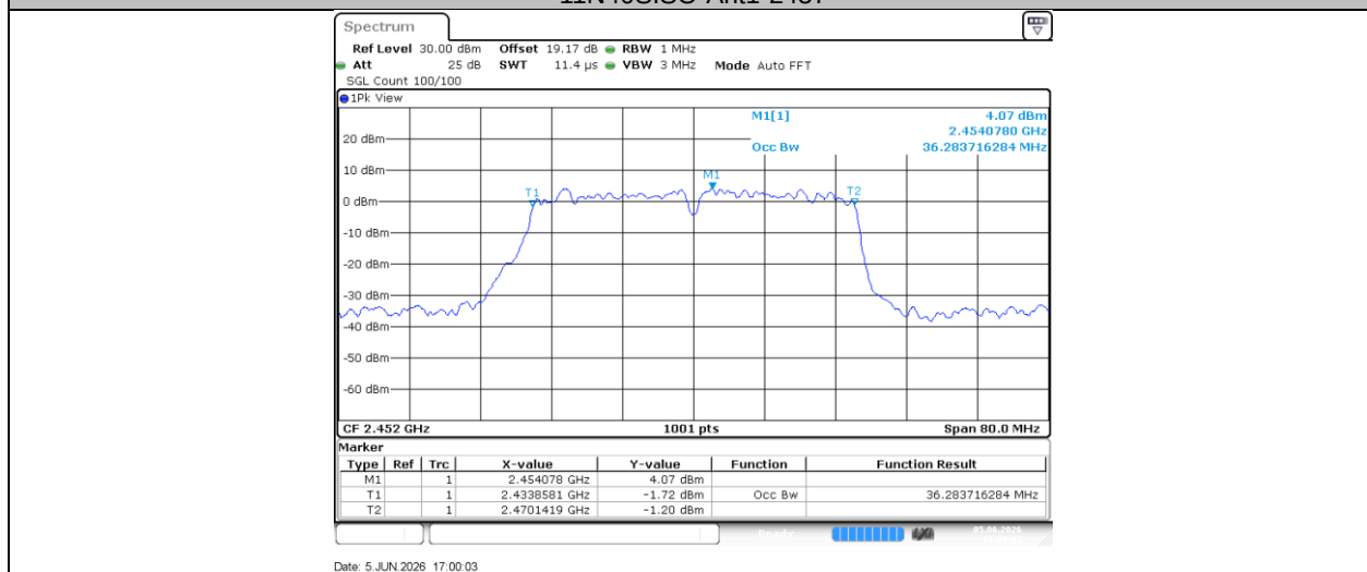
11N40SISO-Ant1-2452
