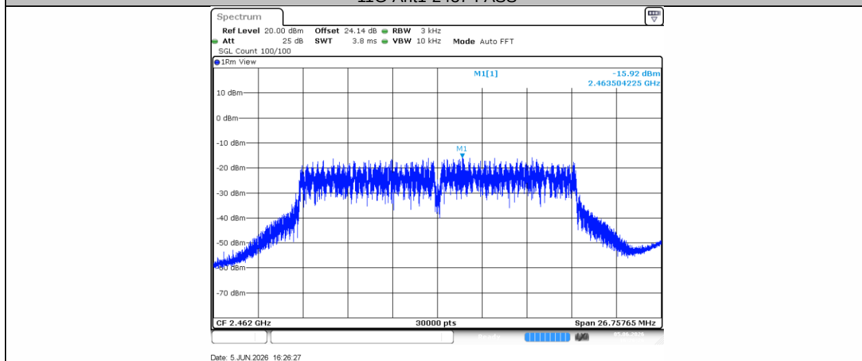
11G-Ant1-2462-PASS
