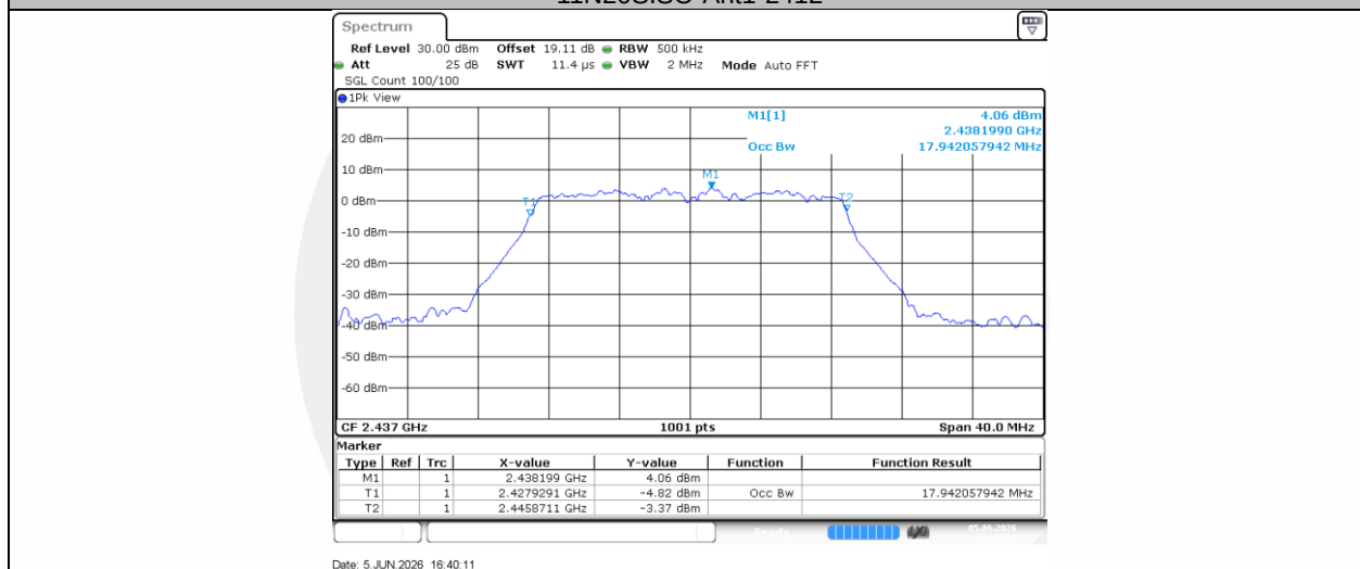
11N20SISO-Ant1-2437
