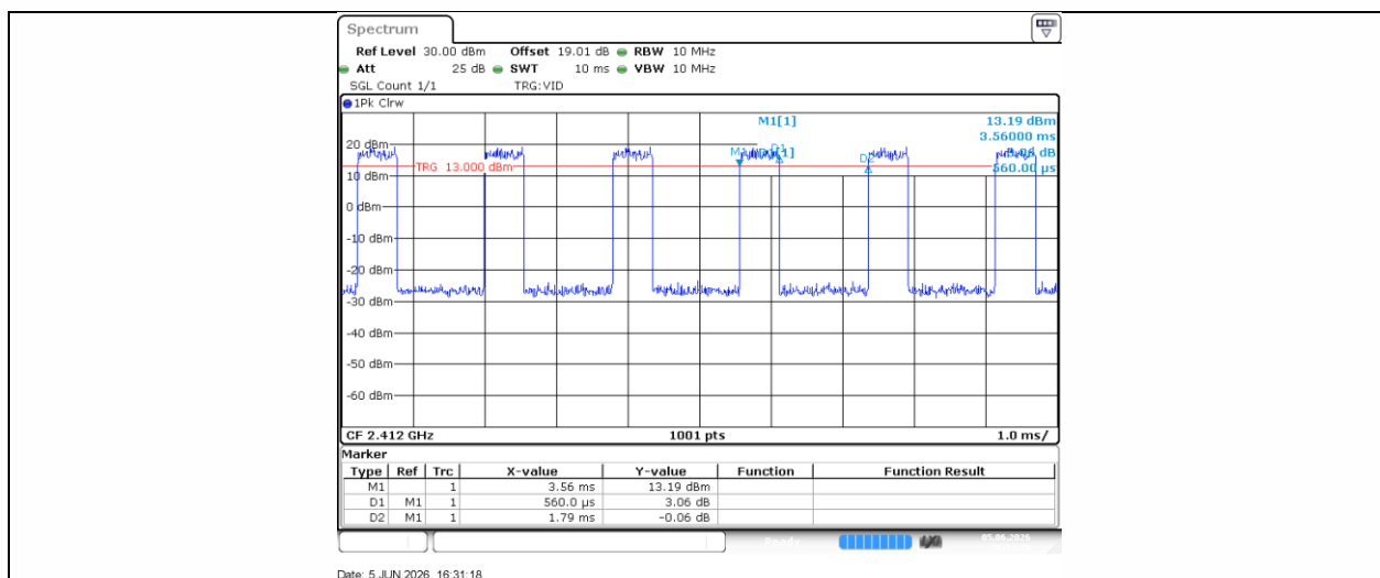
NTNV-11N20SISO-Ant1-2412
