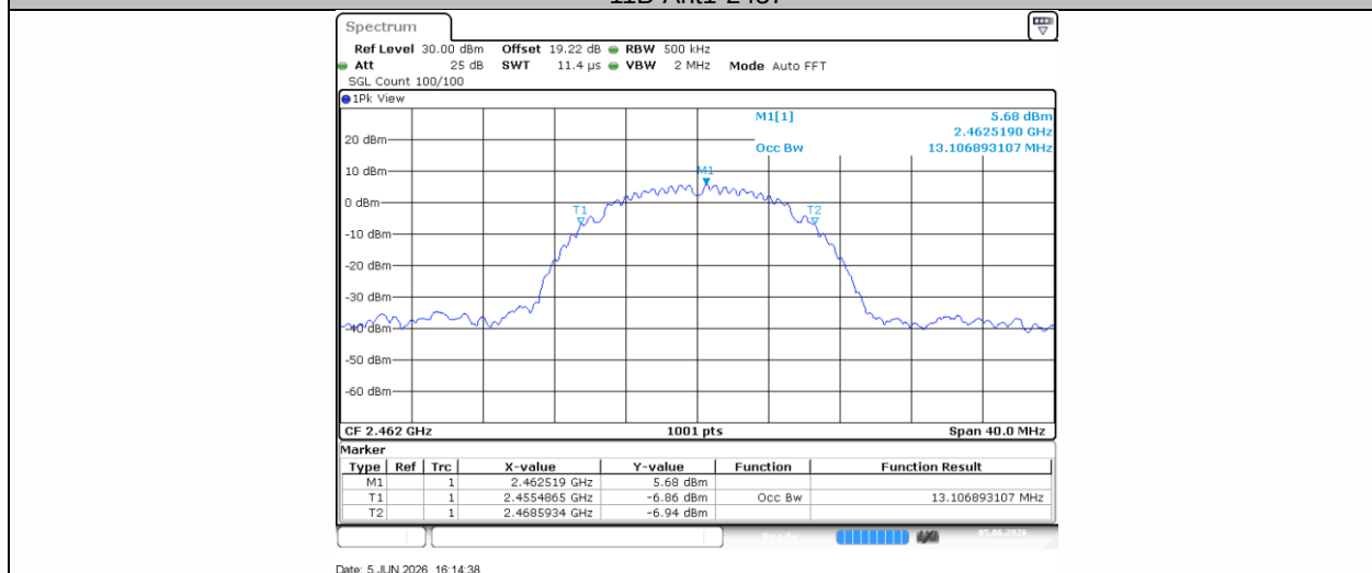
11B-Ant1-2462
