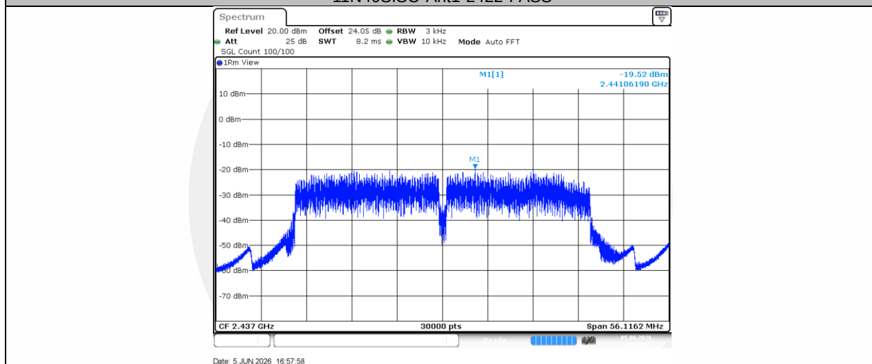
11N40SISO-Ant1-2437-PASS
