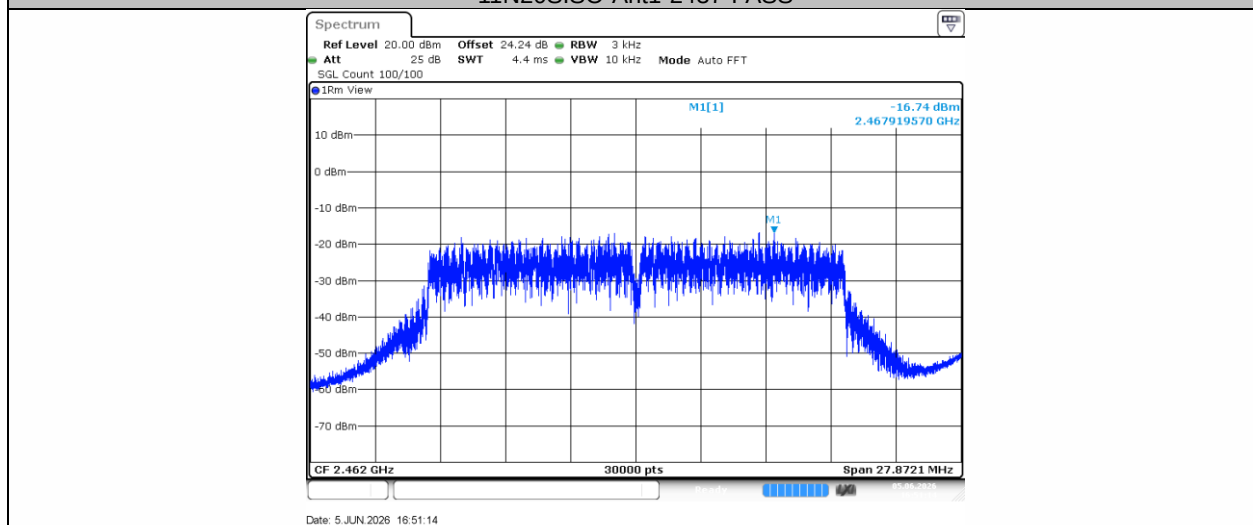
11N20SISO-Ant1-2462-PASS
