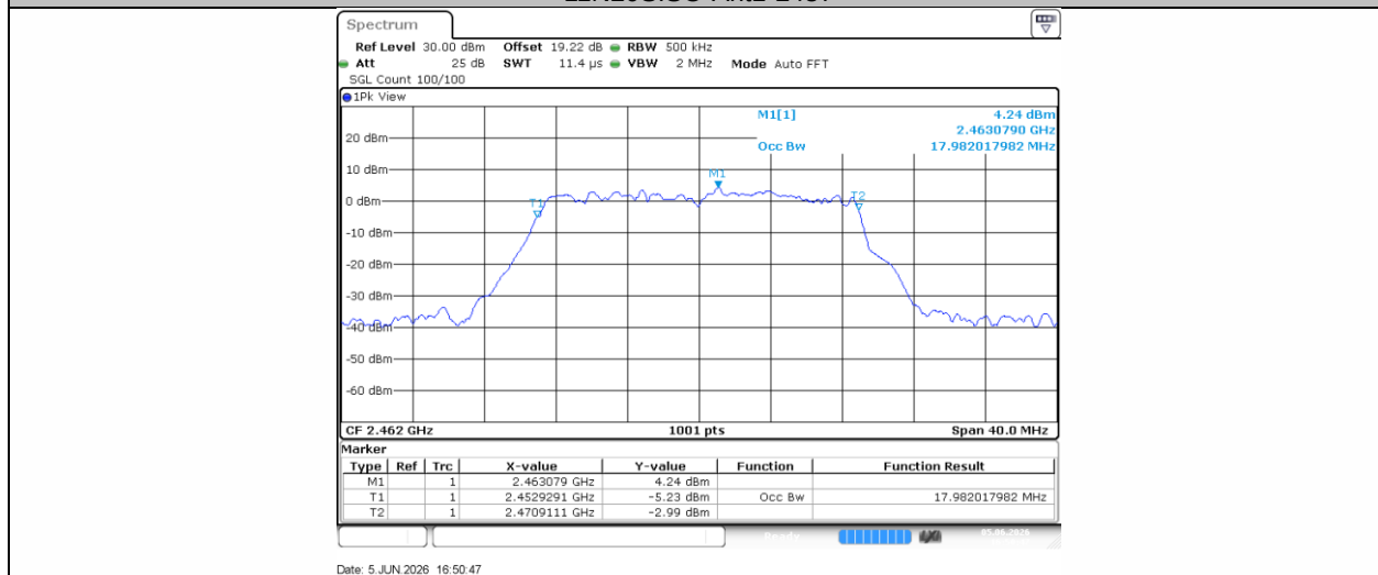
11N20SISO-Ant1-2462
