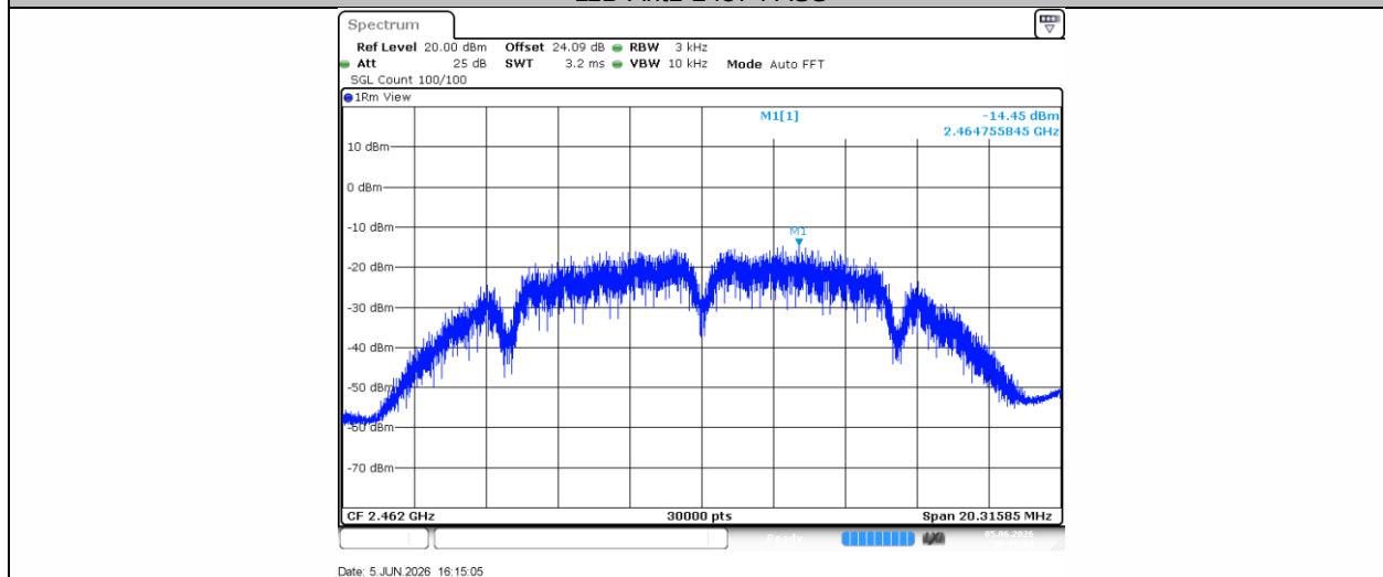
11B-Ant1-2462-PASS
