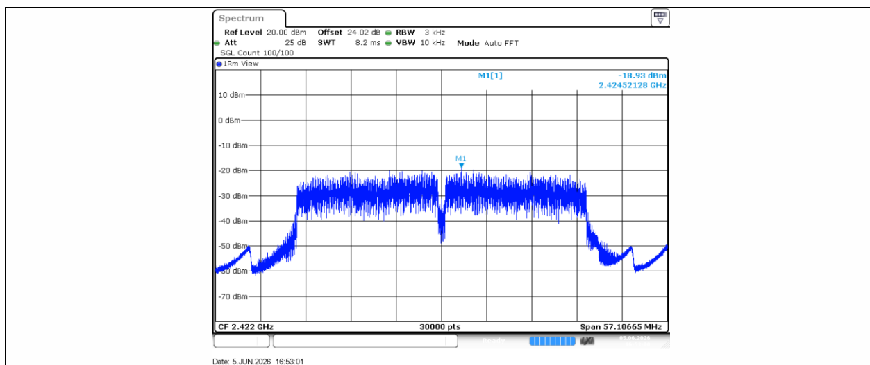
11N40SISO-Ant1-2422-PASS
