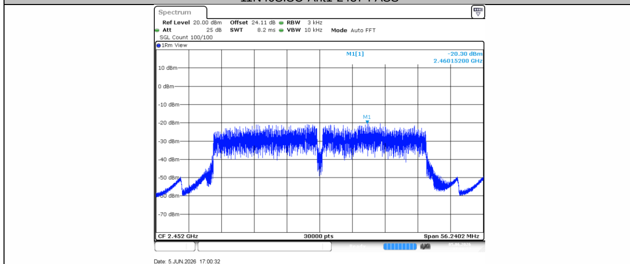
11N40SISO-Ant1-2452-PASS
