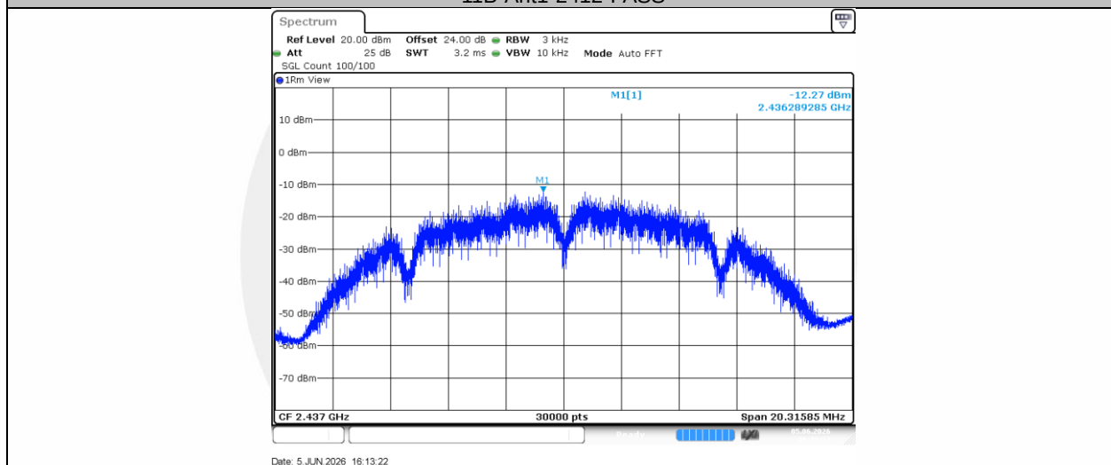
11B-Ant1-2437-PASS
