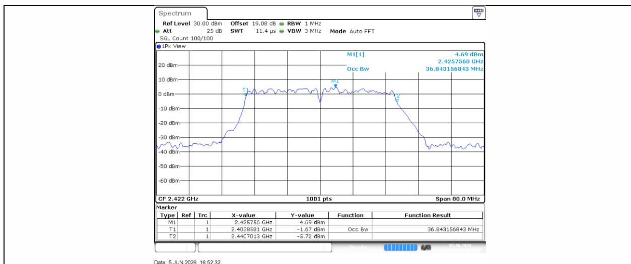
11N40SISO-Ant1-2422
