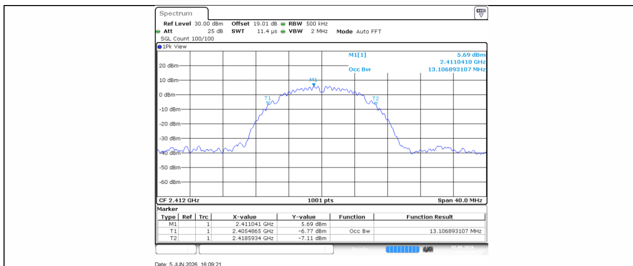
11B-Ant1-2412
