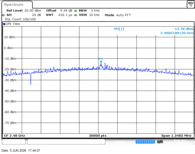
BLE_2M-Ant1-2480-PASS
