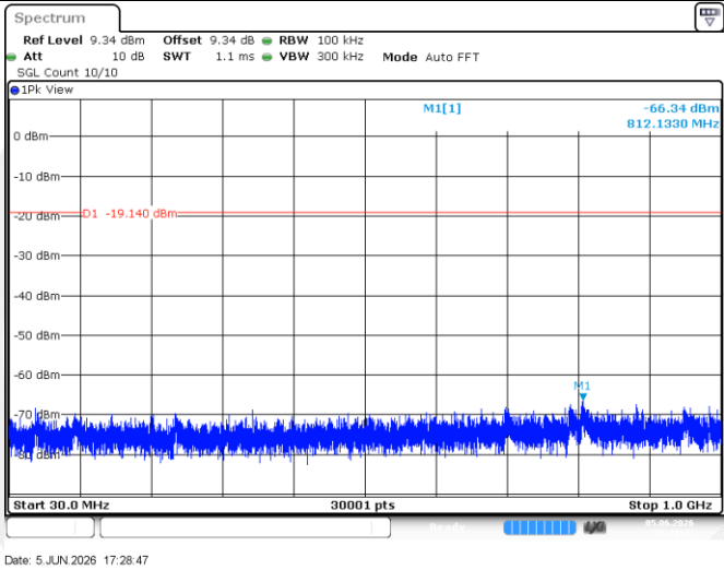
BLE_1M-Ant1-2480-30-1000-PASS
