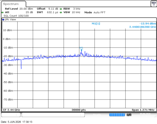
BLE_2M-Ant1-2440-PASS
