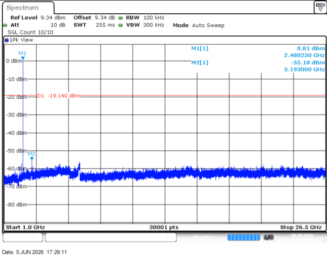
BLE_1M-Ant1-2480-1000-26500-PASS
