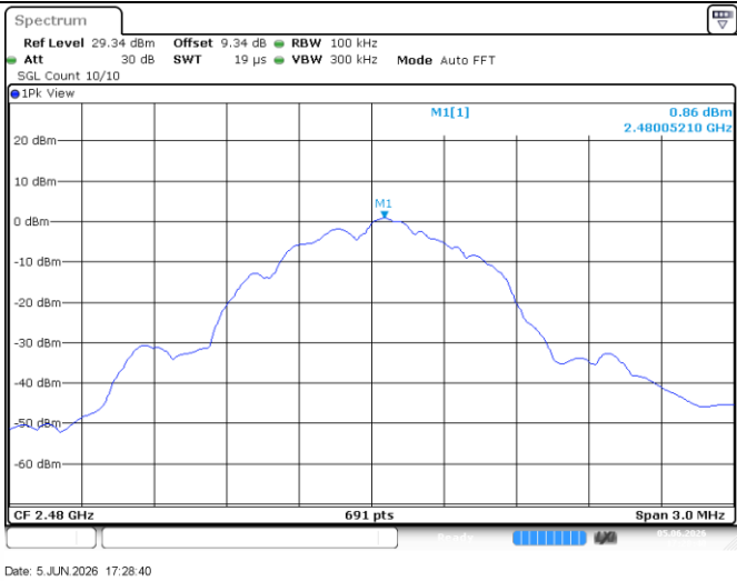
BLE_1M-Ant1-2480-0-Reference-PASS
