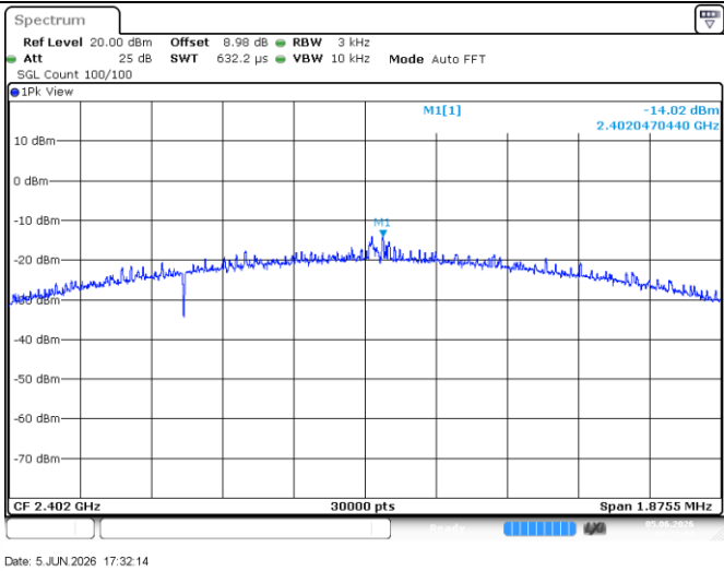
BLE_2M-Ant1-2402-PASS
