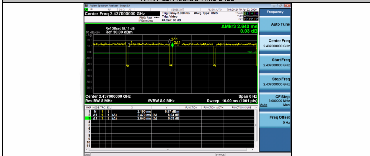
NTNV-11N40SISO-Ant1-2437
