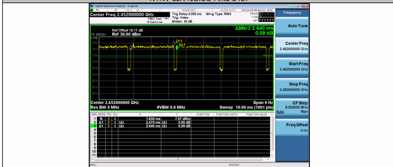
NTNV-11N40SISO-Ant1-2452
