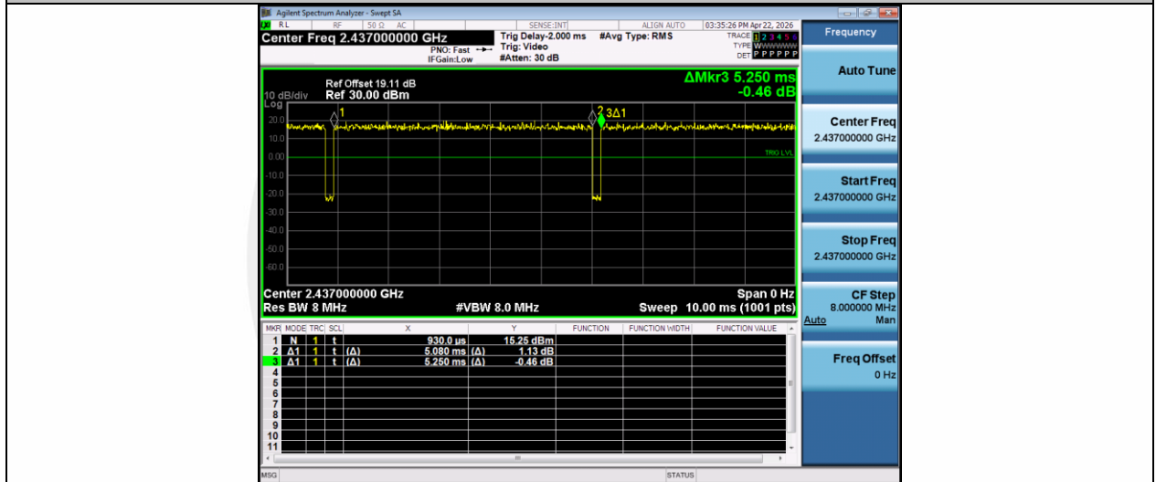
NTNV-11N20SISO-Ant1-2437
