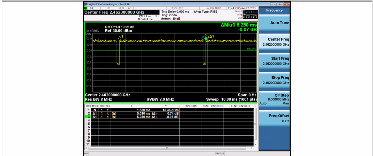
NTNV-11N20SISO-Ant1-2462
