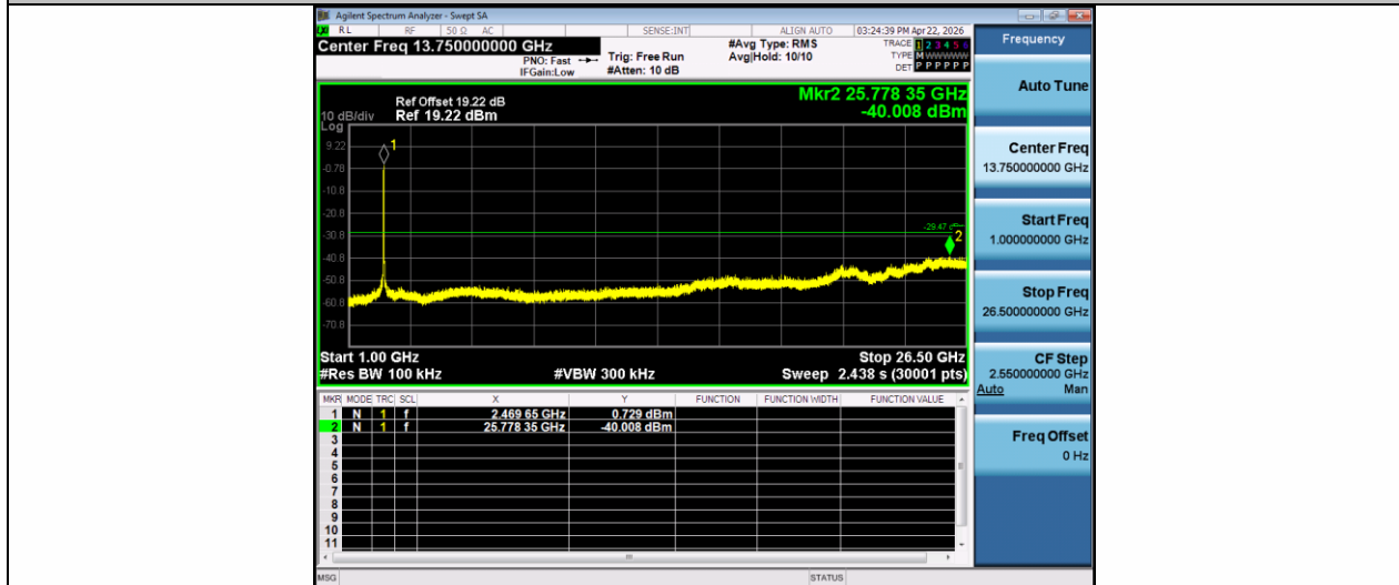
11G-Ant1-2462-1000~26500-PASS
