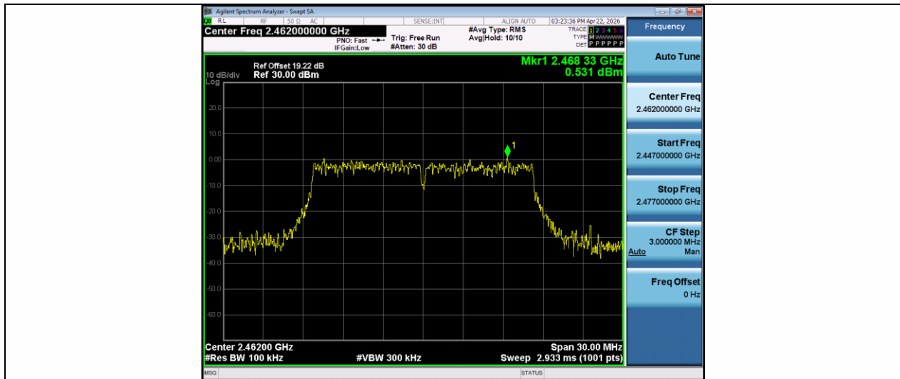
11G-Ant1-2462-0~Reference-PASS
