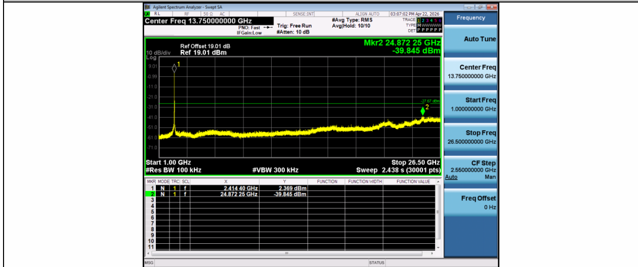
11G-Ant1-2412-1000~26500-PASS
