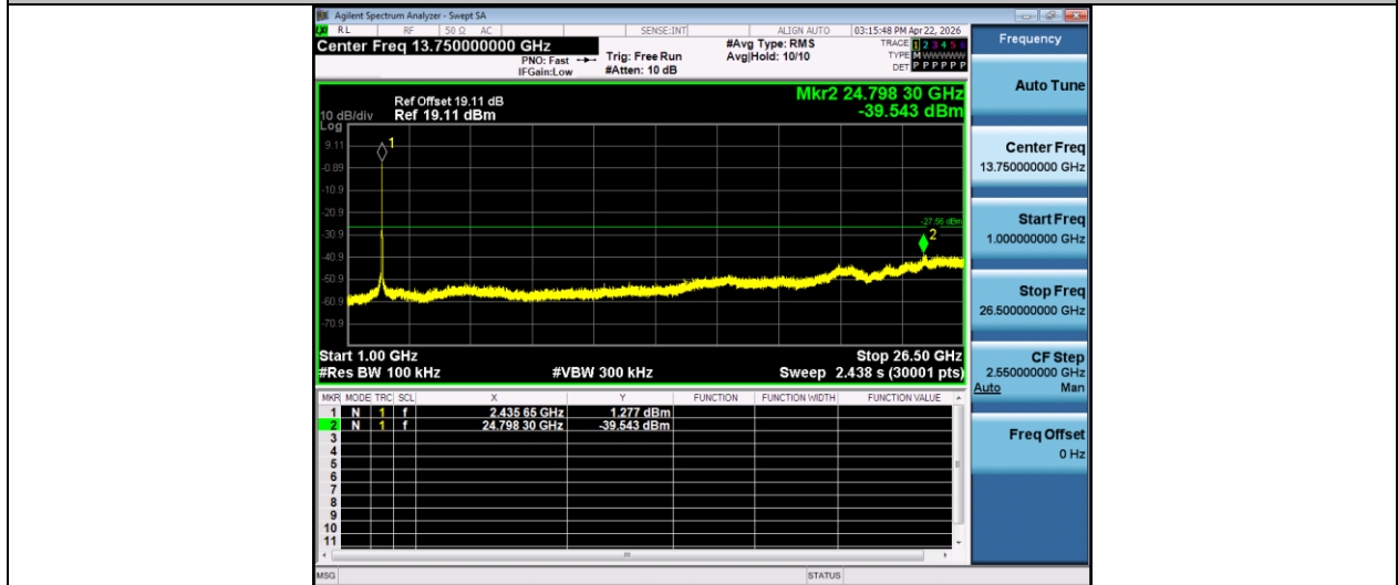
11G-Ant1-2437-1000~26500-PASS
