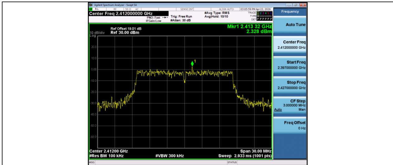
11G-Ant1-2412-0~Reference-PASS
