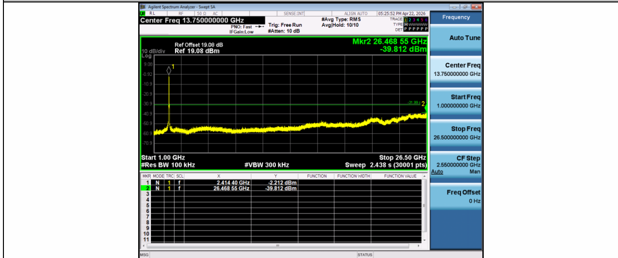
11AX40SISO-Ant1-2422-1000~26500-PASS
