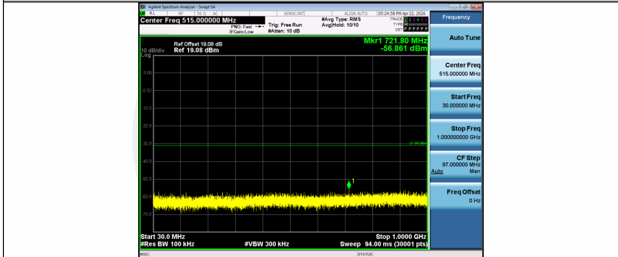
11AX40SISO-Ant1-2422-30~1000-PASS
