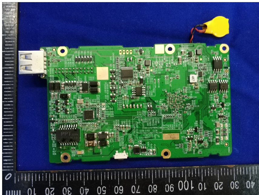
Solder Board-Component View 3
