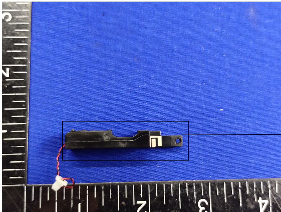
LDS Antenna
